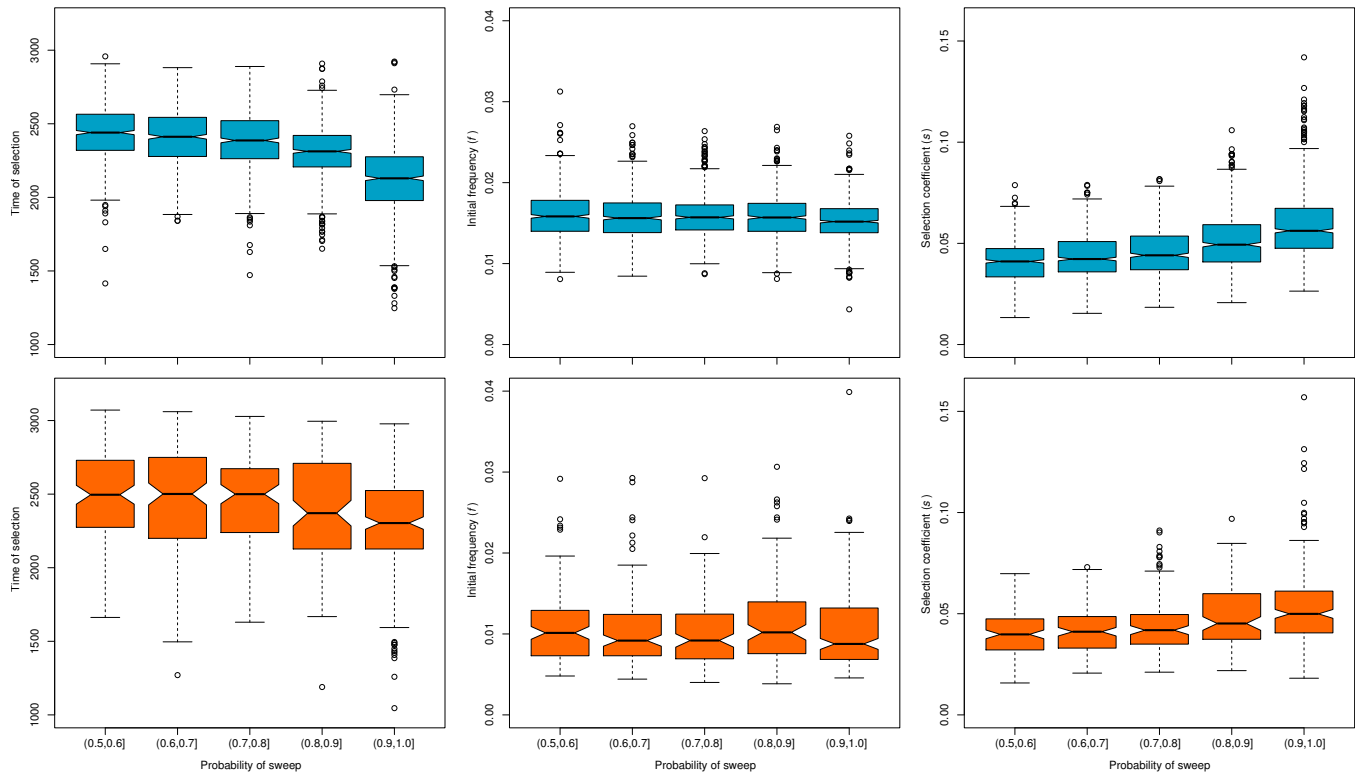
Figure S29: Predicted selection parameters for all genes in YRI (orange) and CEU (blue) with probability of being classified as sweep greater than 0.5 divided into bins of probability of sweep (Left) Predicted number of generations before present at which selection began (Time of selection) as a function of the probability of sweep. (Middle) Frequency reached by mutation before becoming beneficial ( f ) as a function of probability of sweep. (Right) Selection coefficient ( s ) as a function of probability of sweep.
