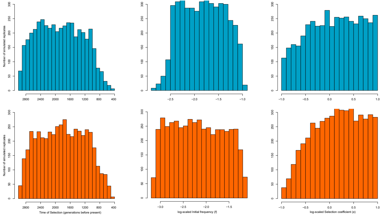
Figure S34: Distribution of selection parameters for simulations of sweeps conducted with demographic history parameters of CEU (top row) and YRI (bottom row). (Left column) Distribution of time at which tracked mutation becomes beneficial (reaches initial frequency) in simulations of selective sweeps. (Middle column) Distribution of log-scaled initial frequency (input parameter) reached by mutation before becoming beneficial in simulations of selective sweeps. (Right column) Distribution of log-scaled selection coefficient in simulations of selective sweep.
