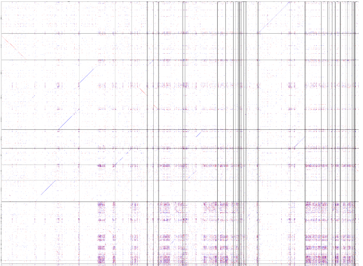
Supplementary Data 7. Dotplot illustrating homology between the current F. oxysporum f. sp. lini assembly (before filtering redundant contigs with the Purge Haplotigs tool) and GCA_003615085.1 / FoC_Fus2_v1 deposited in the NCBI Genome database (vertical axis).
