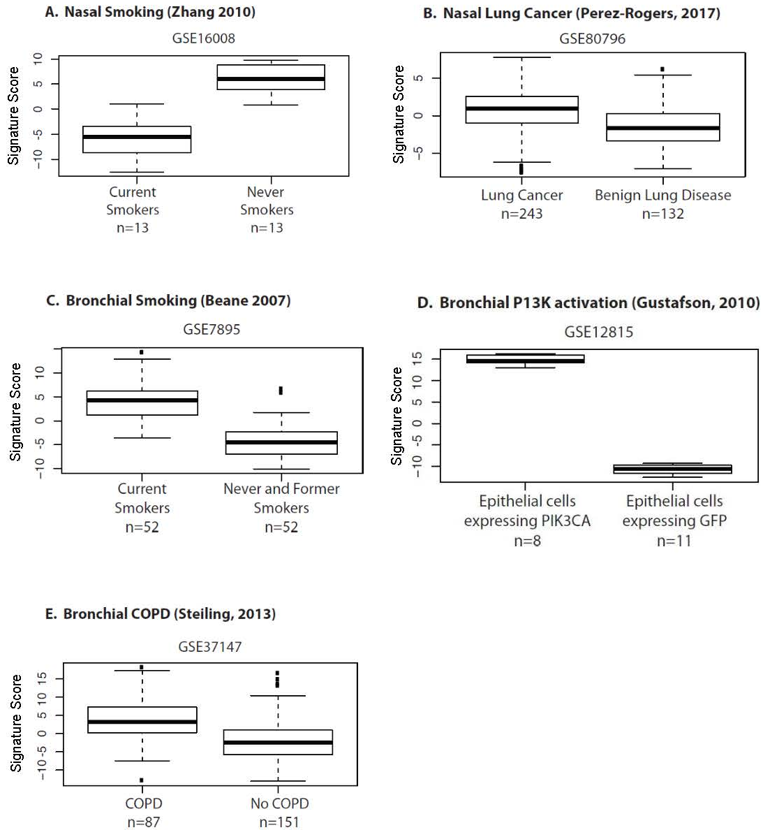
Figure S2: Boxplots of the gene signature scores in the datasets used to derive the gene signatures. (A-E) Boxplots of the signature score for each gene signature of interest detailed in the Supplementary Methods in the datasets in which the gene signature was derived.
