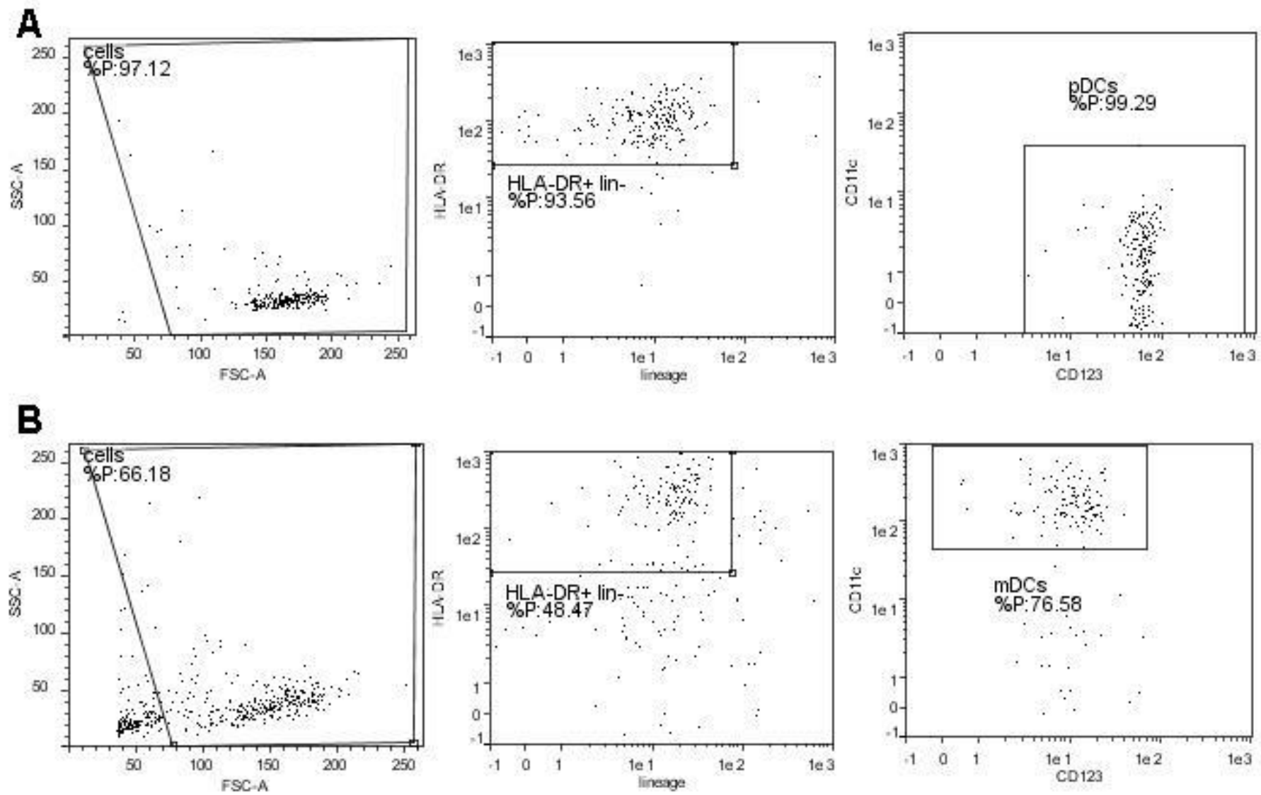
Figure S1. Gating strategy for purity assessment of isolated DCs. pDCs (panel A) are characterized as lin^{-} , HLA-DR ^{+} , CD11c ^{-} and CD123 ^{+} . mDCs (panel B) are characterized as lin^{-} , HLA-DR ^{+} , CD11c ^{+} and CD123 ^{-} .
