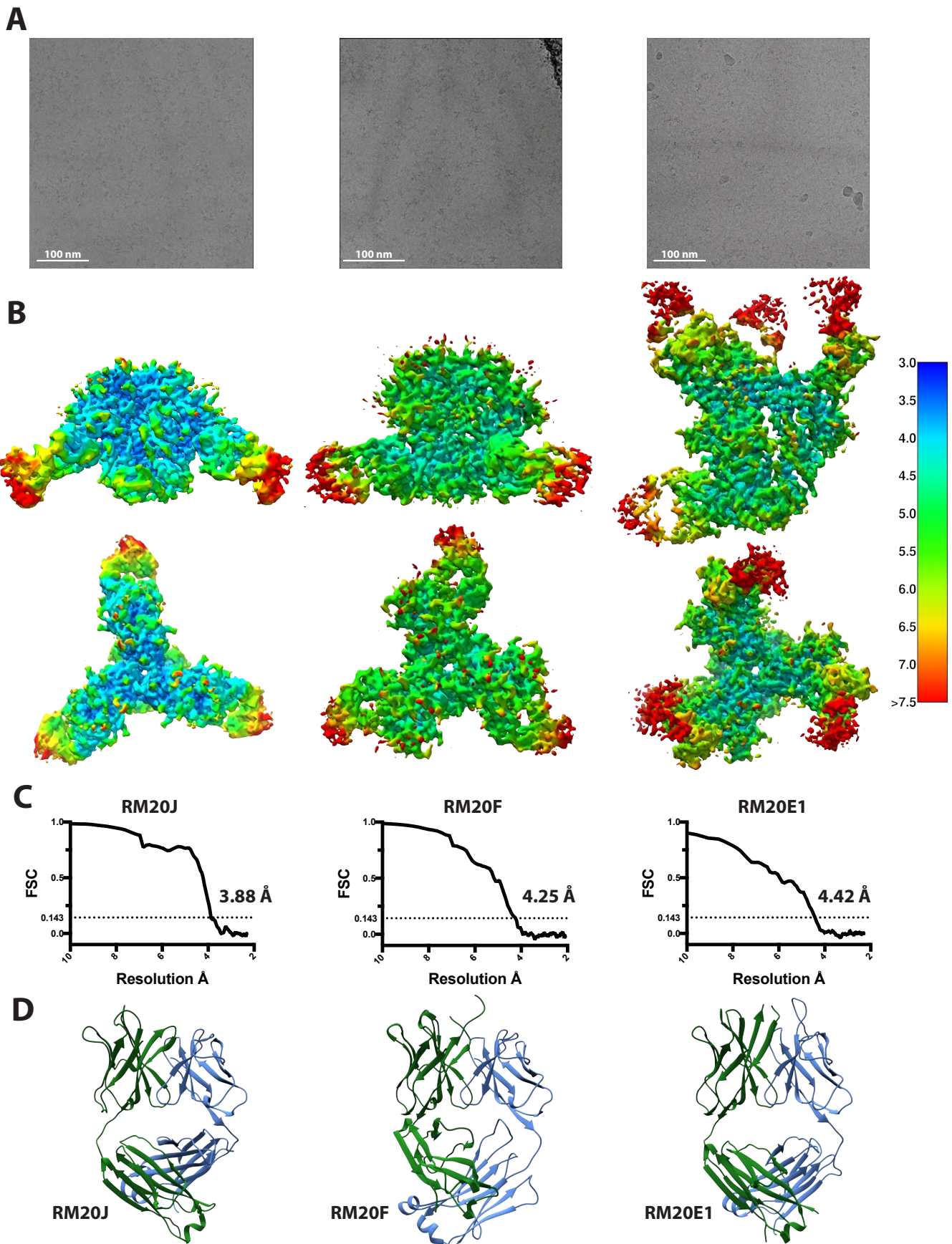
S3 Fig. Cryo-EM structures of BG505 SOSIP trimers with mAbs and crystal structures of mAbs. (A) Representative micrographs for cryoEM datasets. (B) Local resolution maps for each complex generated in cryoSPARC v2 (Punjani et al., 2017). (C) Gold-standard Fourier shell correlation (FSC) curves for each complex showing global resolution calculated at FSC = 0.143. (D) Crystal structures of unliganded Fabs RM20J, RM20F, and RM20E1. Heavy chains are shown in green and light chains shown in light blue.
