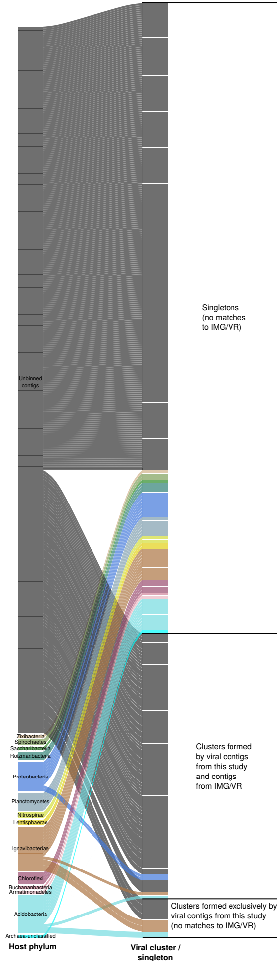
Supplementary Figure S3: Viral clusters and singletons in relation to host taxonomy. The alluvial plot shows the complete set of the 385 detected viral contigs in this study and phylum-level taxonomy of their host, if known. Related Figure 2b shows only a subset of this figure (shows only singletons with assigned host taxonomy and only those clusters which contained some contigs with assigned host taxonomy).
