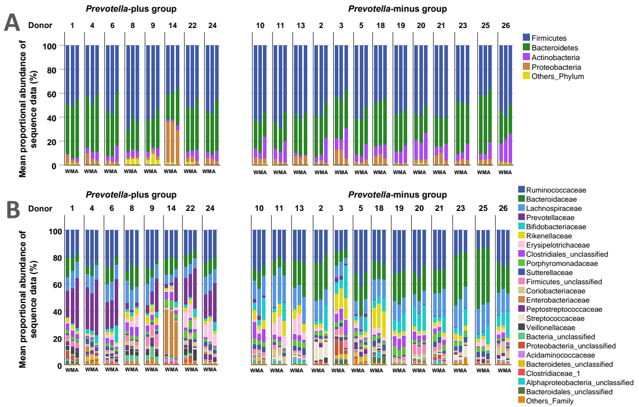
Additional file 5: Figure S1. Changes in average proportional abundance within individual volunteers at the bacterial (A) phylum and (B) family level based on Illumina MiSeq sequencing of 16S rRNA gene amplicons. W= washout period, M= Maltodextrin period, A= AXOS period.
