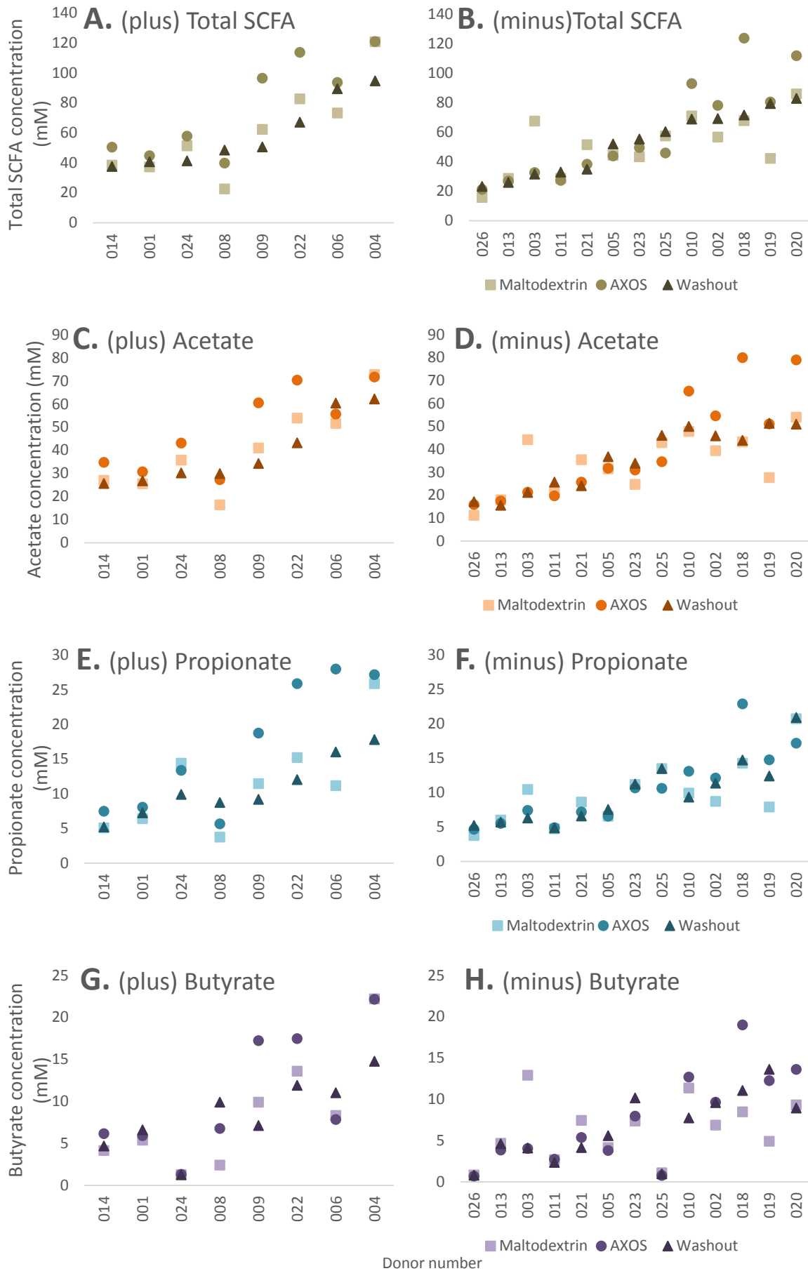
Additional file 8: Figure S3. Concentration of short chain fatty acids in faecal samples from the washout, maltodextrin and AXOS periods for both the Prevotella - plus and Prevotella - minus group, showing (A, B) total SCFA, (C, D) acetate, (E, F) propionate and (G, H) butyrate.
