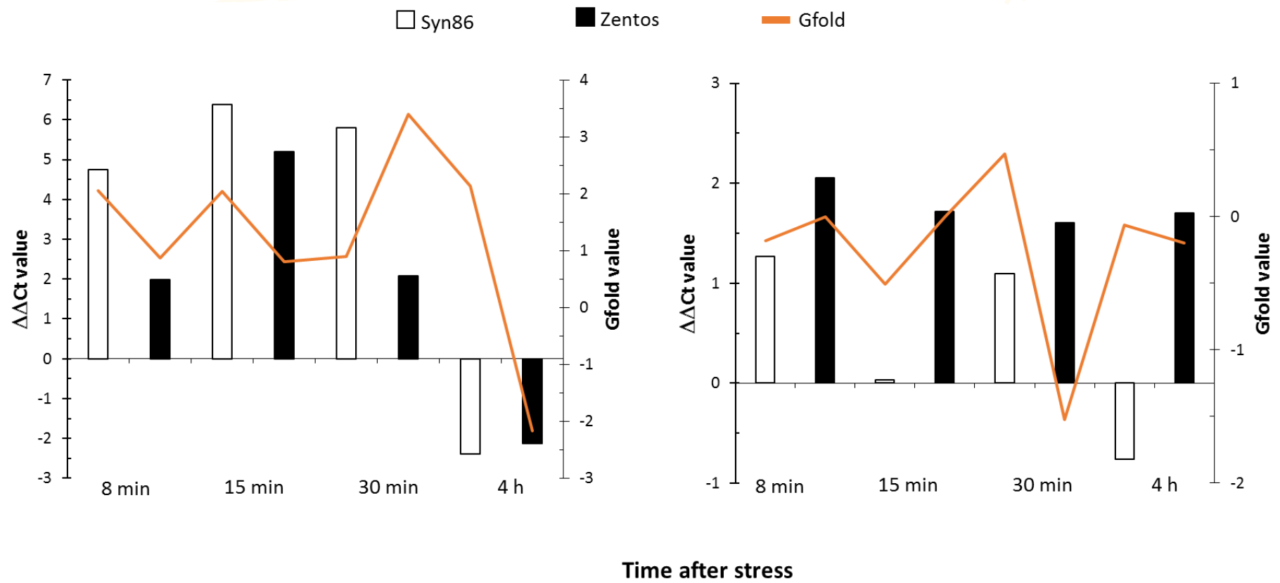
Fig. S4. Comparison of GFOLD values and \Delta\Delta Ct values of TraesCS5D02G238700 and TraesCS2D02G173600 in Syn86 and Zentos.
