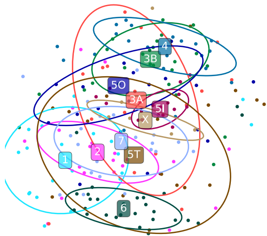
Bipolar cells
