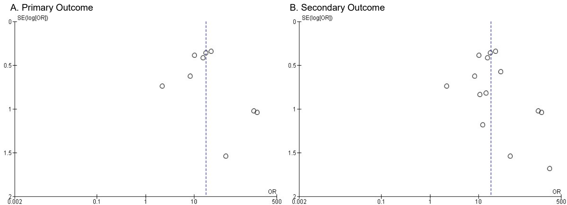
Supplementary Figure S1. Funnel Plots of Studies Included in the Primary (A) and Secondary Outcomes (B) Analysis. The distribution of effect sizes of studies included in both analyses were distributed symmetrically.
