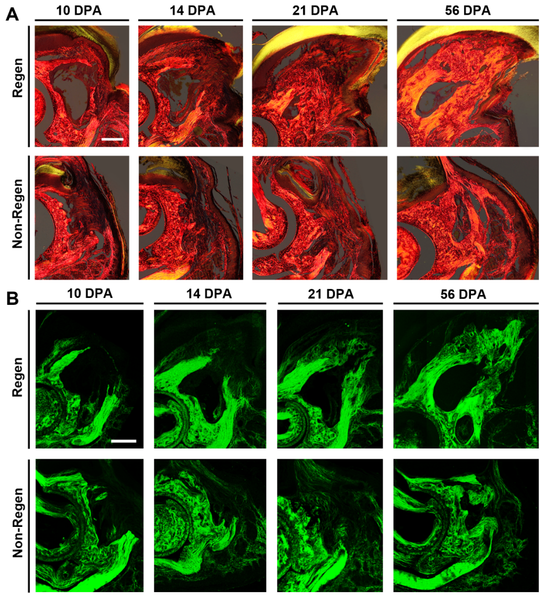
Fig. S2. Time course of bone and fibrous tissue regeneration. (A) Picosirius Red (PSR) staining visualized with polarized light microscopy and (B) second harmonic generation (SHG) imaging at various DPA show collagen fibers aligned proximodistally and dorsoventrally in Regen and Non-Regen digits, respectively. Bone regrowth occurs only in the Regen group. Scale: 0.2 mm.
