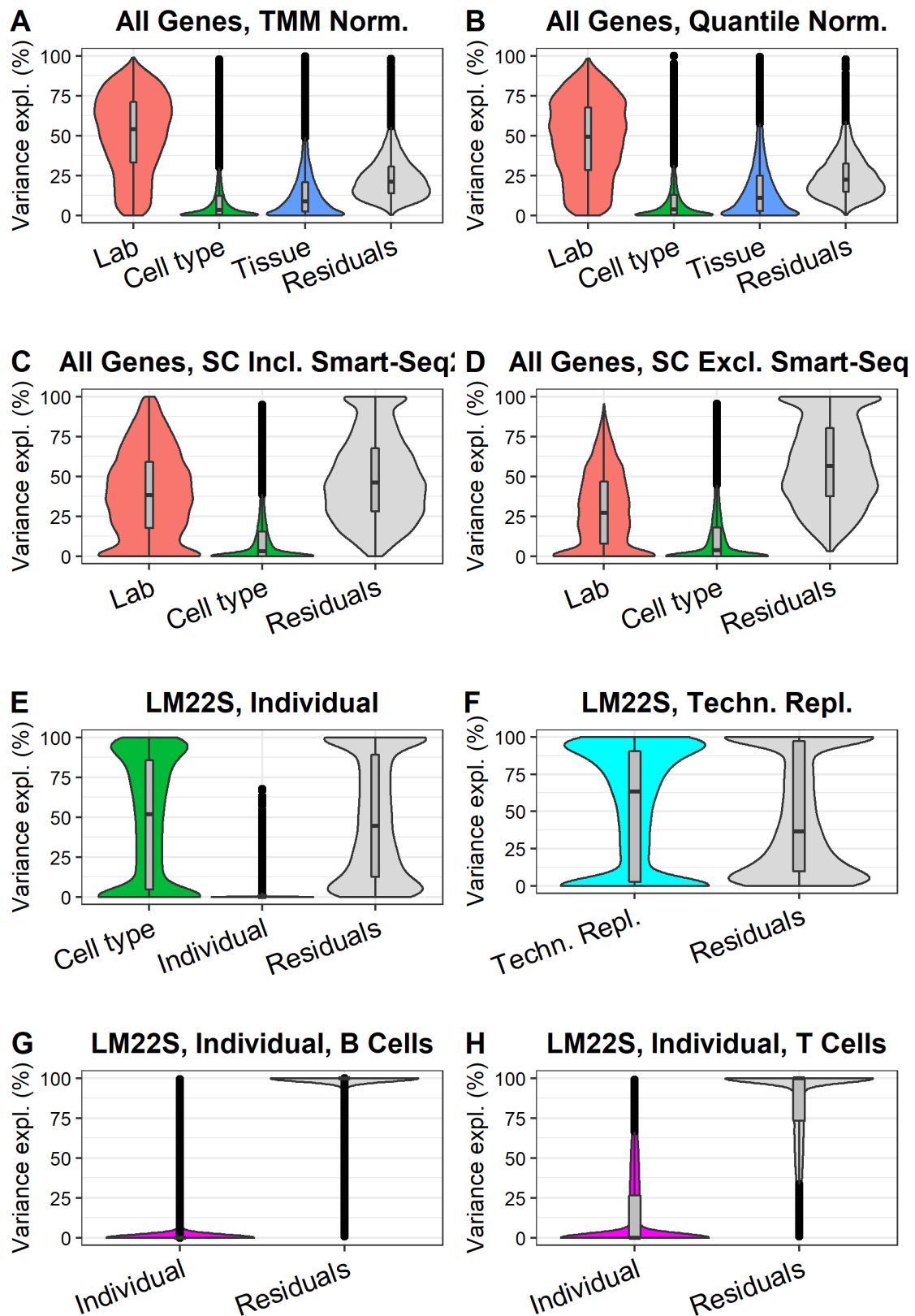
Fig. S4. Additional plots for explained variance. A, B: Comparison between TMM and Quantile Normalization. C-D: The effect of including Smart-Seq2 samples. E. Variance explained by having samples from different individuals compared to samples from the same individual but taken at different time points. F. Variance explained by having different samples compared to technical replicates, where the same sample has been sequenced several times. G, H. Same data as E, but separated on cell type into two groups to make individual factor more comparable to the technical replicates shown in F.
