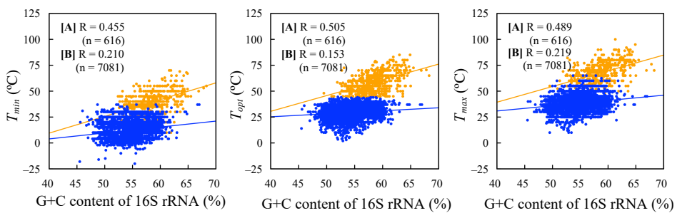
Fig. S1. Correlations between the G+C content of 16S rRNA and each growth temperature ( T_{min} , T_{opt} , and T_{max} ) in thermophilic and hyperthermophilic ([A], orange, and orange line), and the other bacterial strains ([B], blue circle, and blue line). Correlation was determined using the Pearson correlation coefficients (R values).
