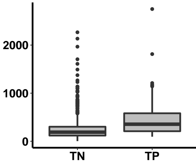
exp_mis p = 2e-17
