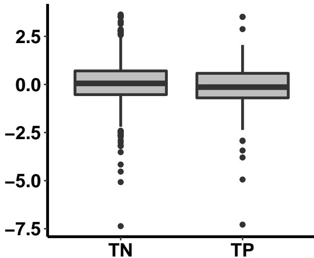
syn_z p = 2e-01
