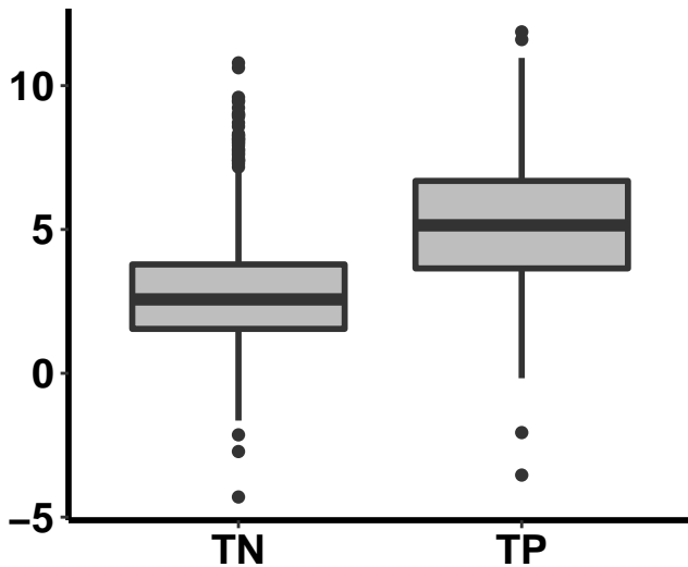
lof_z p = 2e-23
