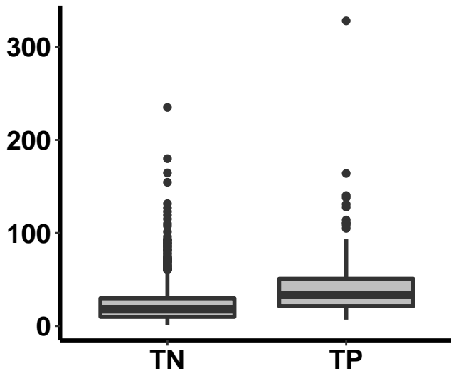
exp_lof p = 6e-17
