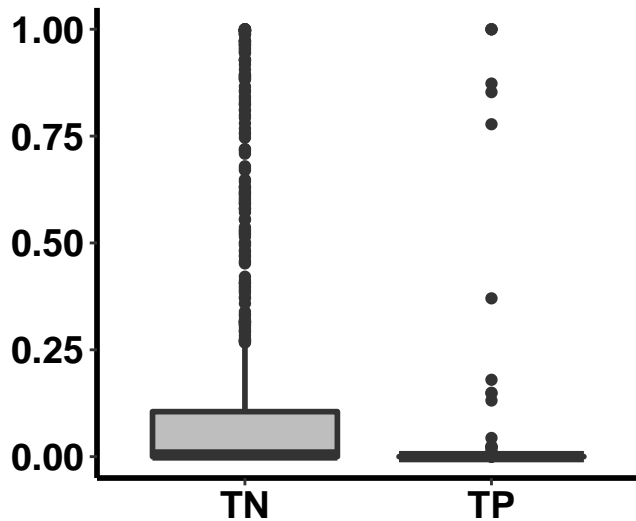
pNull p = 3e-24
