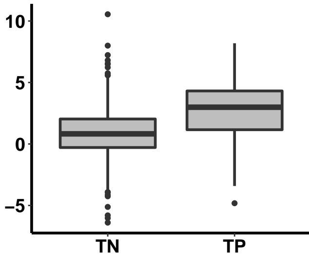
mis_z p = 7e-16
