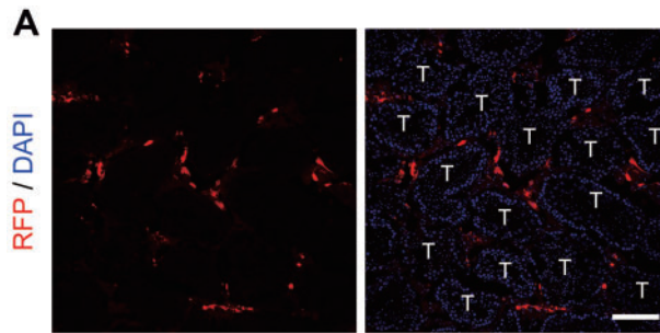
Supplementary Figure S6. Localization of transplanted endosialin + cells in the testes of recipient mice. (A) Immunostaining showed the accumulation of RFP + cells in the testicular interstitium of recipient mice at 4 weeks after transplantation (n = 3). The nuclei were counterstained with DAPI. The scale bar denotes 100 \mu m.
