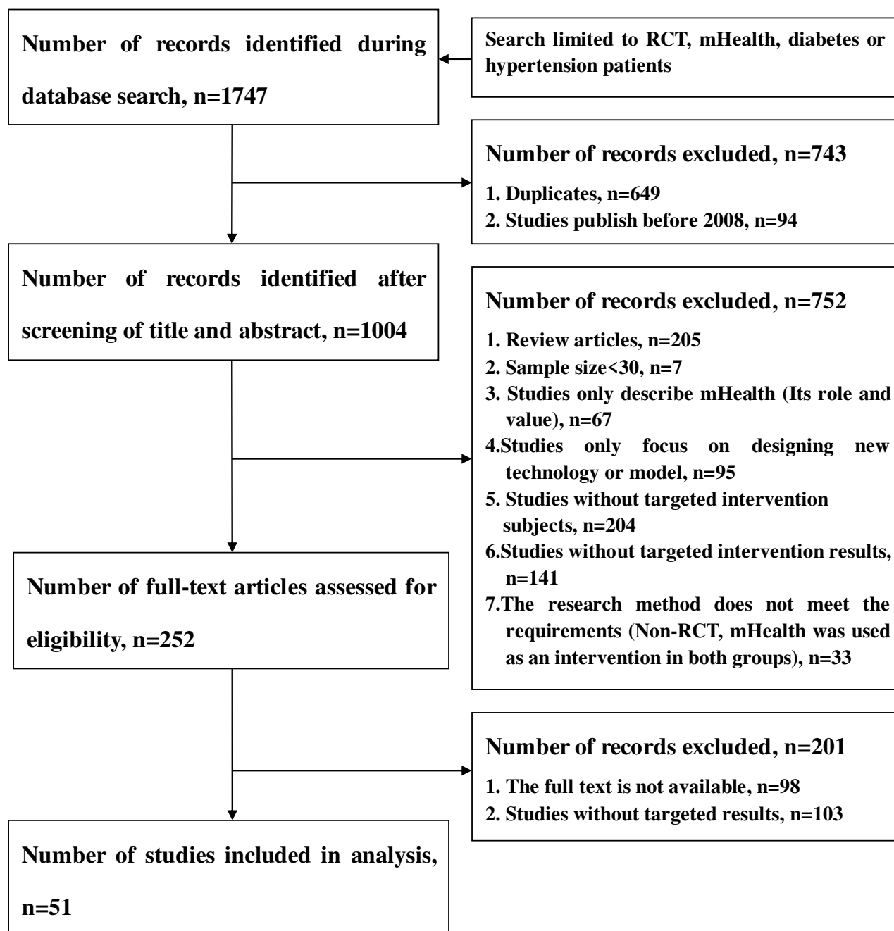
Figure 1 Flow chart of the literature search and study selection procedures
