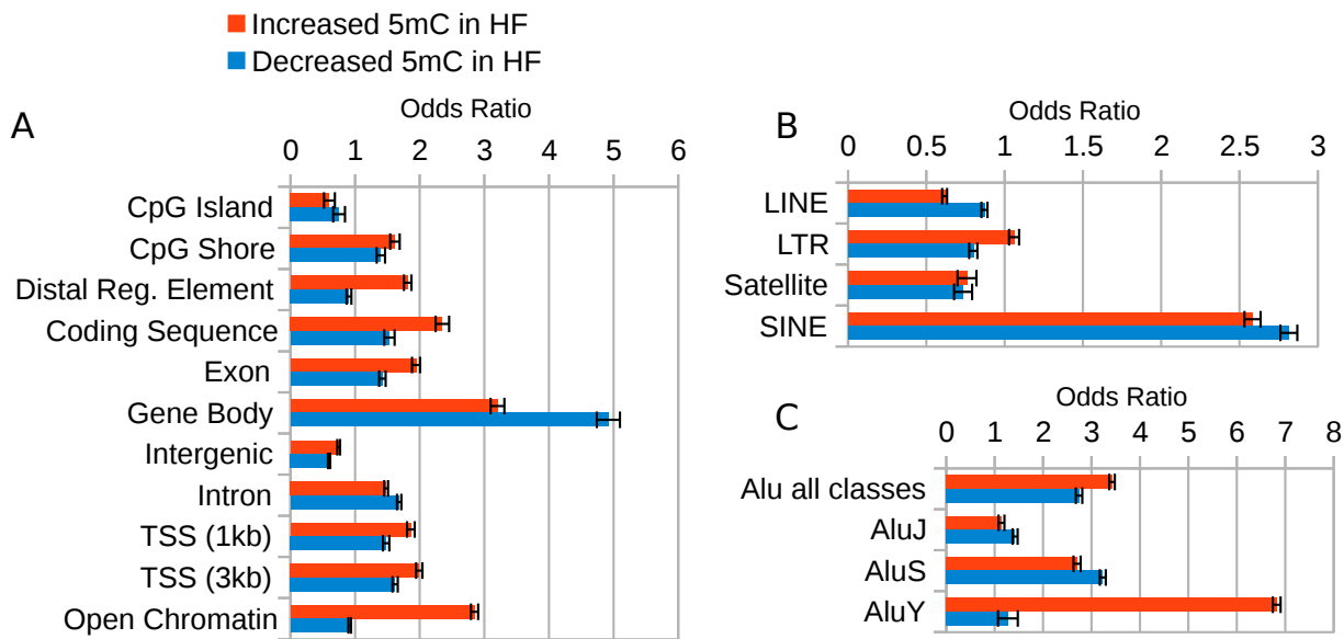
Figure S1. Differential methylation enriched in genomic compartments. Regions with differential methylation (nom p-val<0.01) were intersected with various annotated functional compartments (A), major repeat element classes (B), and Alu subclasses (C).
