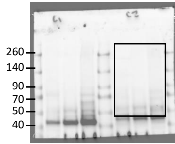
Flag: IP hnRNP-C2
