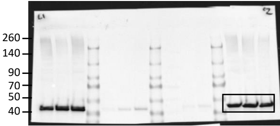
Flag: input hnRNP-C2
