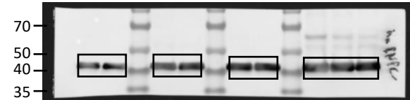
hnRNP-C: HeLa | U2OS | A549 | HEK293
