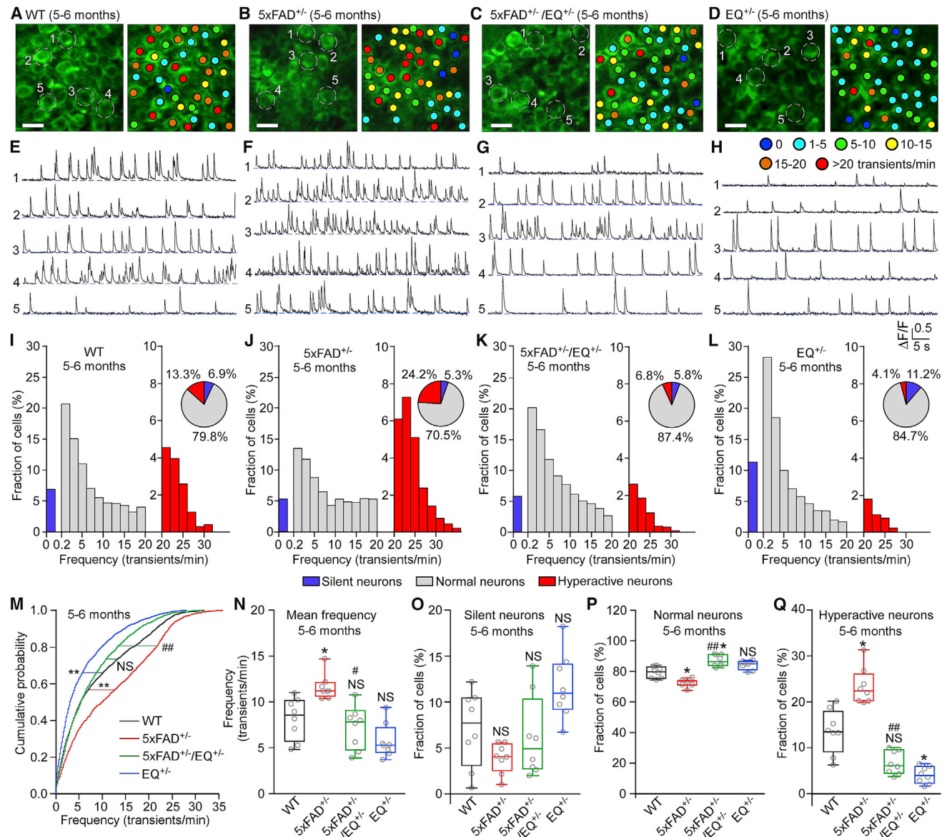
Figure 2. RyR2-E4872Q +/- Prevents Neuronal Hyperactivity of 5x FAD +/- Hippocampal CA1 Neurons In Vivo
