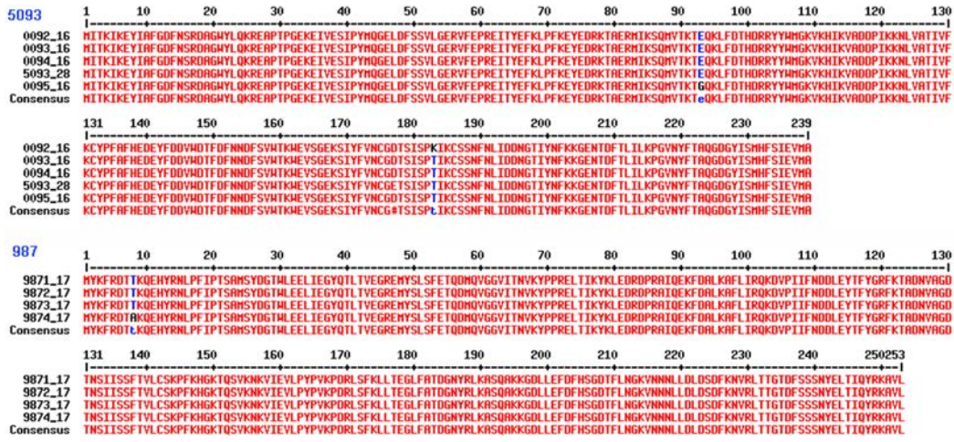
Figure S1. Sequence alignment of the cos (A), pac (Brussowvirus) (B), 5093 and 987 (C) Dit proteins. The conserved amino acids are in red and the partially conserved in blue. Otherwise in black.
