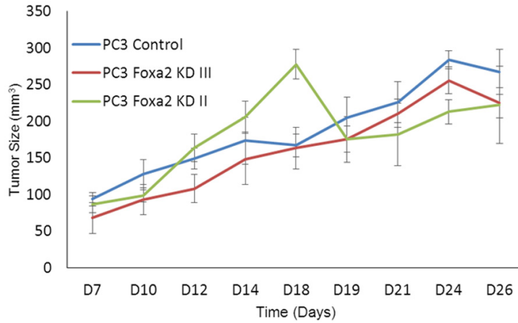
Supplementary Figure 1. PC3/Control and PC3/FOXA2-KD cells were inoculated subcutaneously in mice. The tumor size was measured one-week post-injection, 3 times/week. No statistically significant changes were observed in the tumor growth among the experimental groups. Error bars reported as standard deviation.
