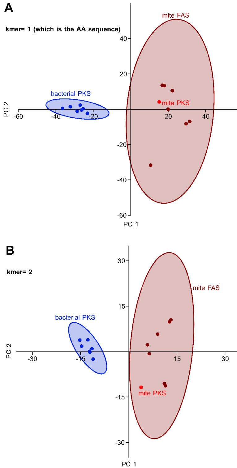
Figure S5. Principle component analyses of the kmer-counting matrices for (a) kmer=1, which equals the amino acid sequence and (b) kmer=2. In both cases the mite sequences including the mite polyketide synthase (red; PKS) were distinctly different from the bacterial PKS (blue). Ellipses represent the 95% confidence.
