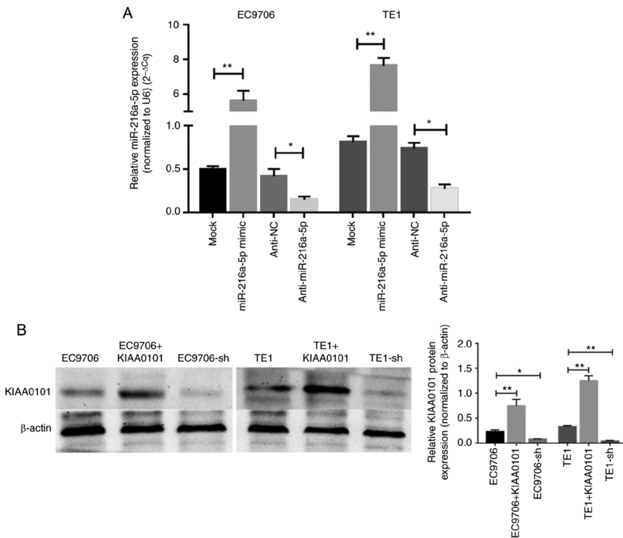
Figure S1. Confirmation of the transfections. (A) The transfections of the miR-216a-5p mimic and anti-miR-216a-5p were confirmed by RT-PCR. * P < 0.05 , ** P < 0.01 . (B) The transfection with KIAA0101 alone (+KIAA0101) increased the protein expression of KIAA0101 in EC9706 and TE1 cells, while transfection with the KIAA0101-targeted shRNA (-sh) decreased the expression of KIAA0101.
