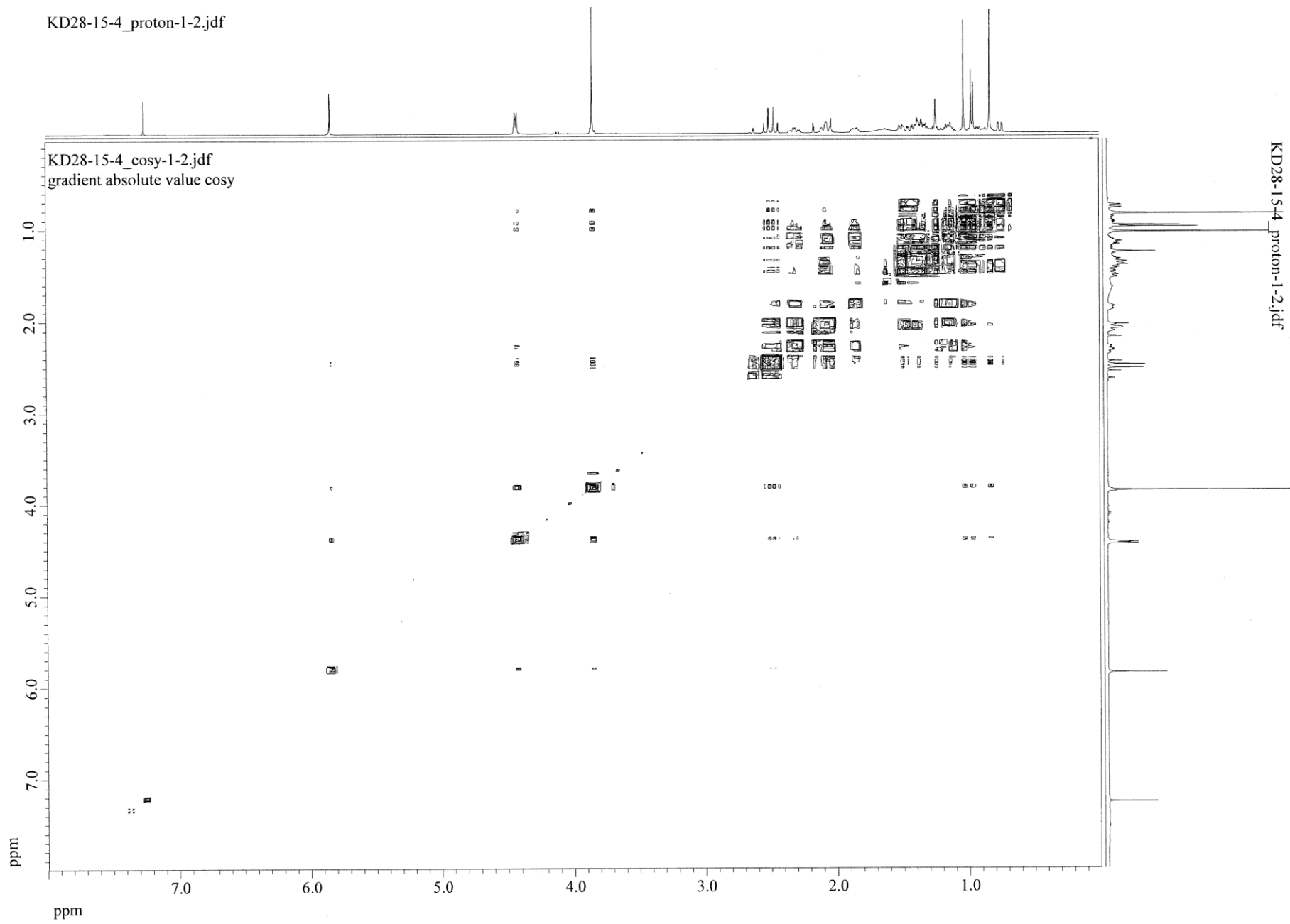
S5. ^1\text{H} - ^1\text{H} COSY spectrum of ilimaquinone in \text{CDCl}_3 .
