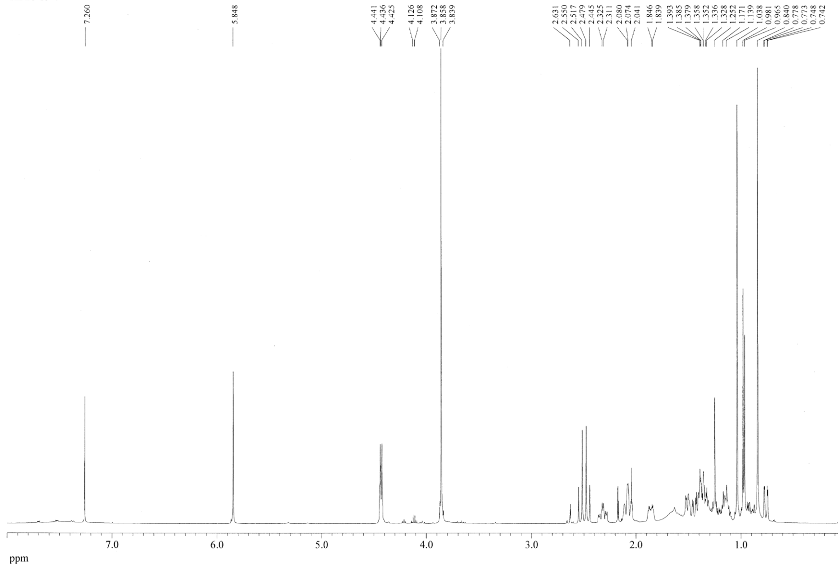
S1. ^1\text{H} NMR spectrum of ilimaquinone in \text{CDCl}_3 at 400 MHz.
