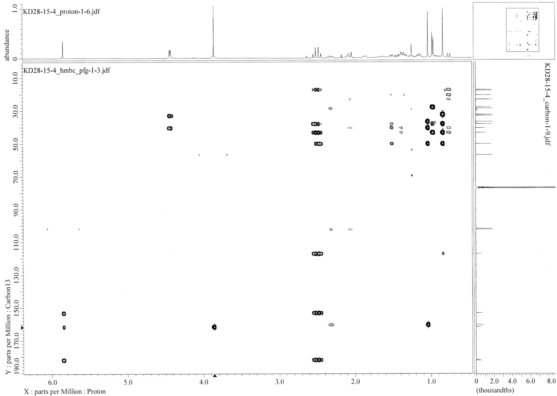
S4. HMBC spectrum of ilimaquinone in CDCl 3 .
