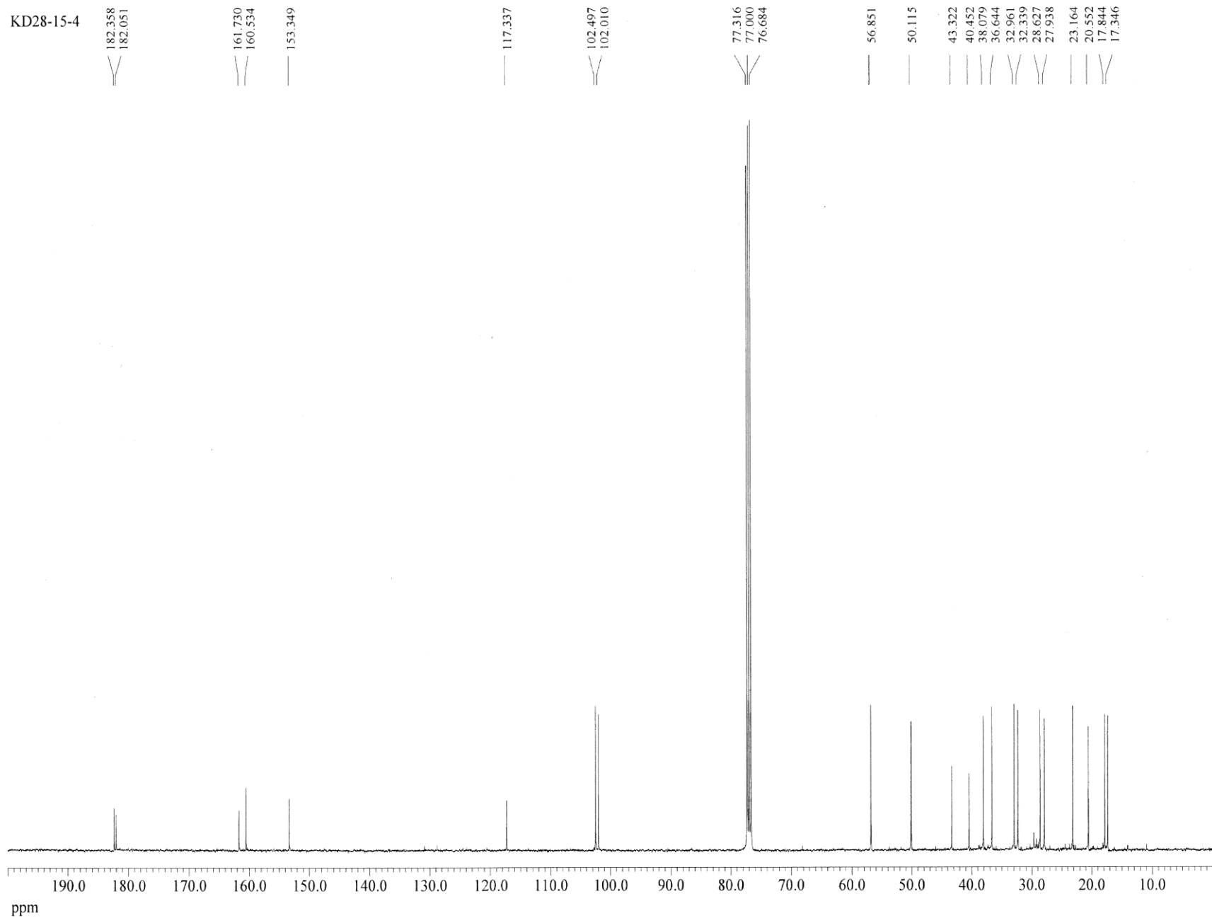
S2. ^{13}\text{C} NMR spectrum of ilimaquinone in \text{CDCl}_3 at 100 MHz.
