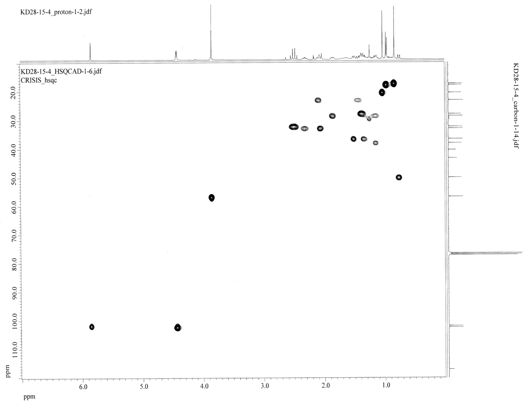
S3. HSQC spectrum of ilimaquinone in \text{CDCl}_3 .
