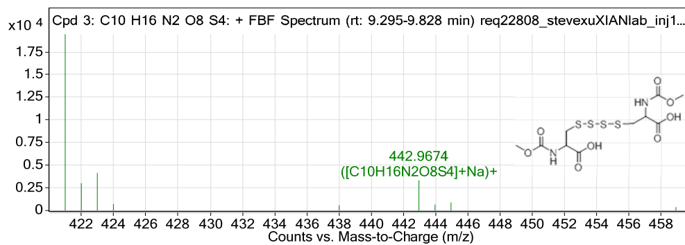
Supplementary Figure 2 PSCP (2 mM) was dissolved in buffer (PBS, 7.4) and incubated under room temperature for 6 h. The resultant mixture was directly analyzed by MS spectrometry.
