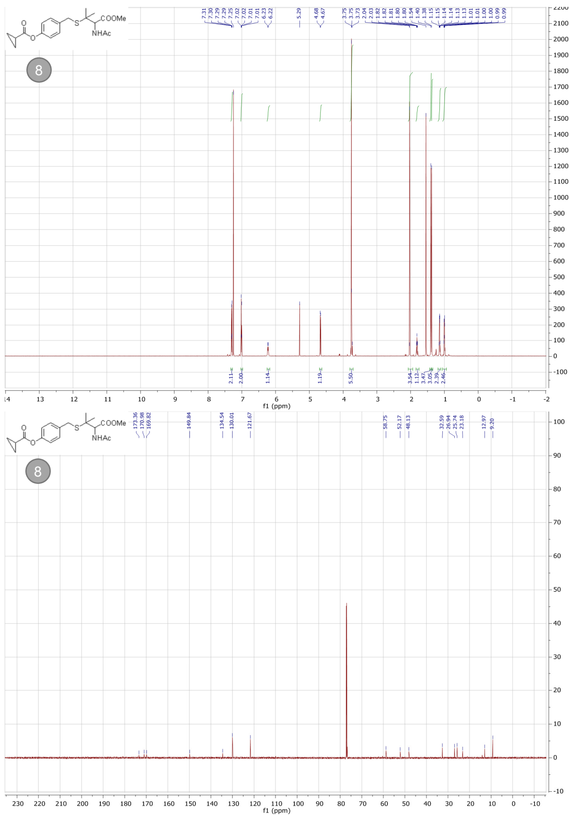
Supplementary Figure 3 Analysis of controllable sulfane sulfur donors (1, 3 5, and 7) and their control compounds (2, 4 6, and 8) using MS spectrometry
