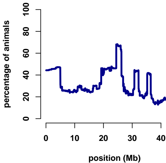
chromosome 24
