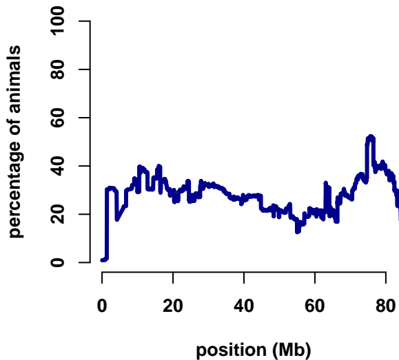
chromosome 2
