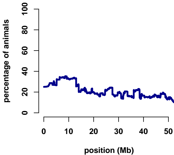
chromosome 23
