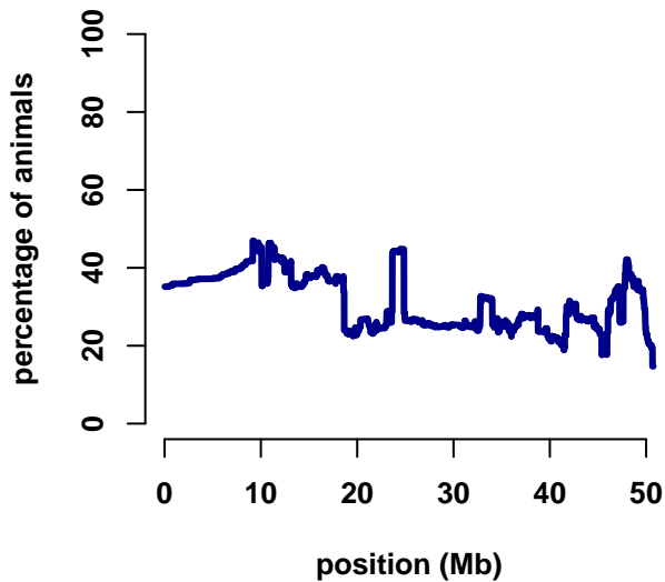
chromosome 21
