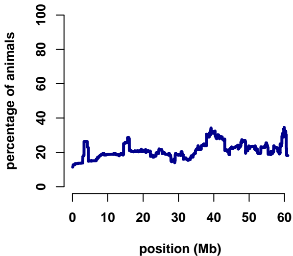
chromosome 14
