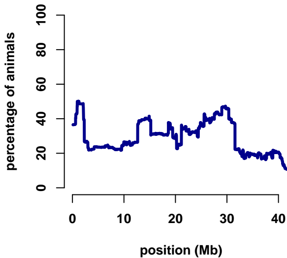
chromosome 34
