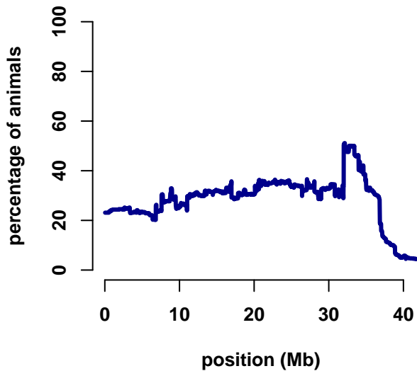
chromosome 29
