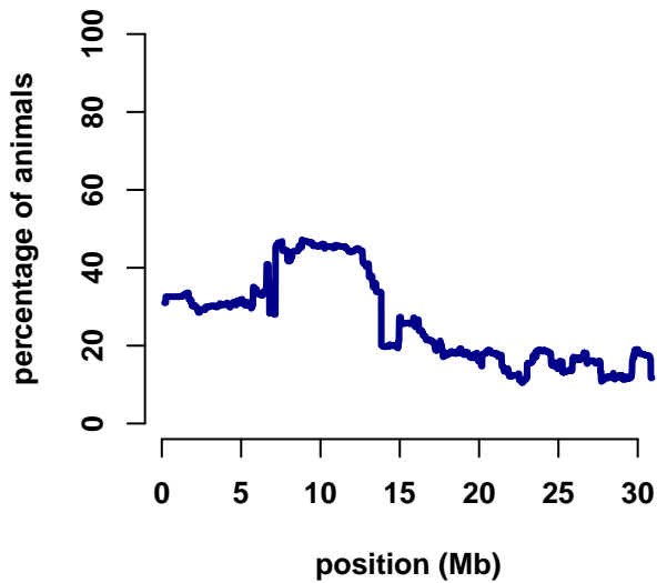
chromosome 37
