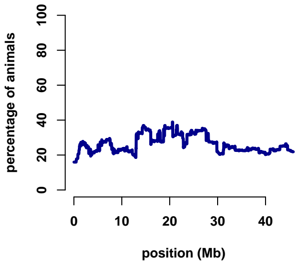
chromosome 27
