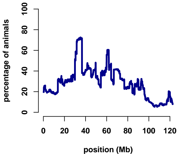
chromosome 1
