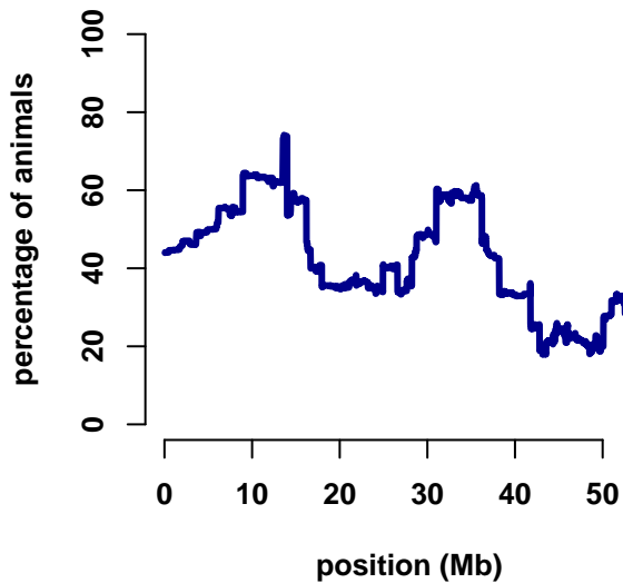
chromosome 18
