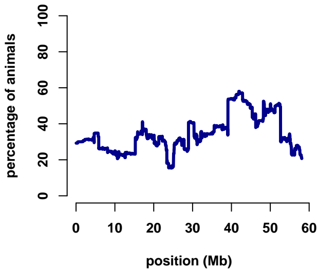
chromosome 20
