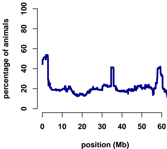
chromosome 13
