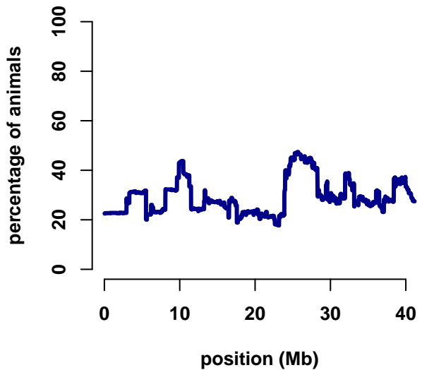
chromosome 28
