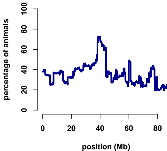
chromosome 4
