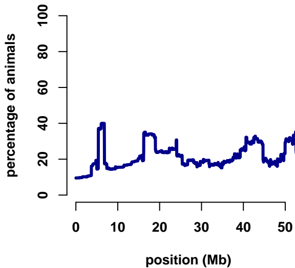
chromosome 19
