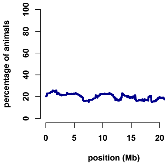
chromosome 38
