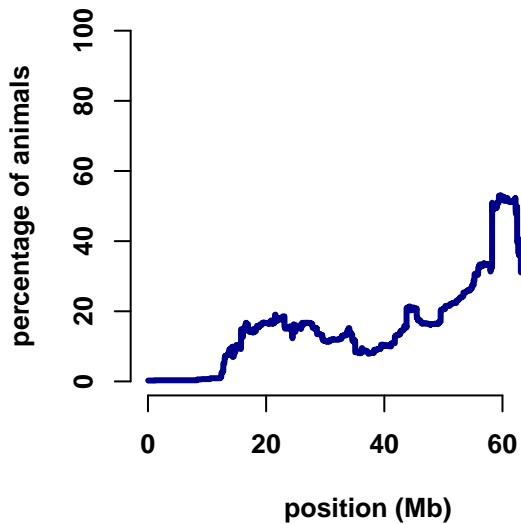
chromosome 11
