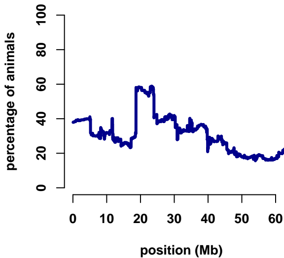
chromosome 17
