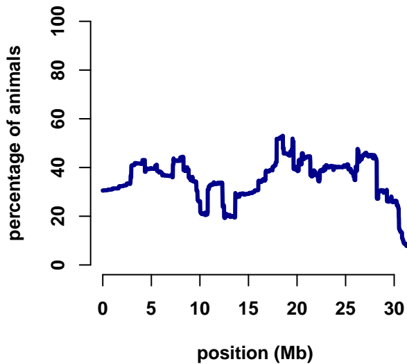
chromosome 33
