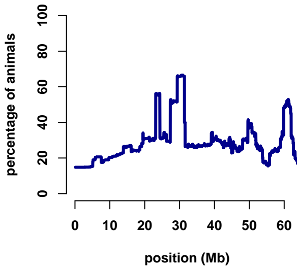
chromosome 15
