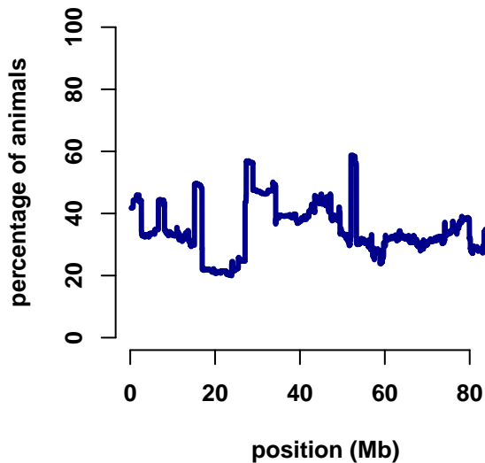
chromosome 3
