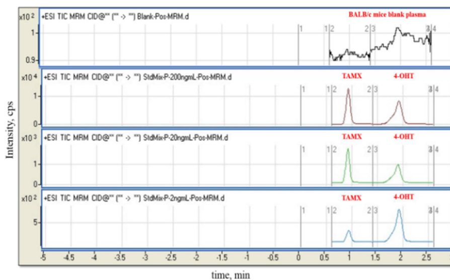
Figure S1. Typical MRM chromatograms of TAMX and 4-OHT in BALB/c mice plasma at three different concentrations (200, 20 and 2 ng/ml) of TAMX and 4-OHT spiked in the mice plasma compared against blank plasma.
