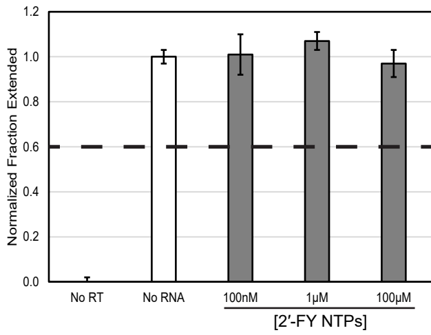
Figure S6 No Effect of 2'-FY Nucleotide Triphosphates on RT Inhibition. Quantification of primer extension assays showing fraction of primer converted into full-length product in control reactions in the absence of RT (No RT) or in the absence of RNA inhibitor (No RNA) and in reactions containing varying concentrations of 2'-FY nucleotide triphosphates (NTPs) (n = 4).
