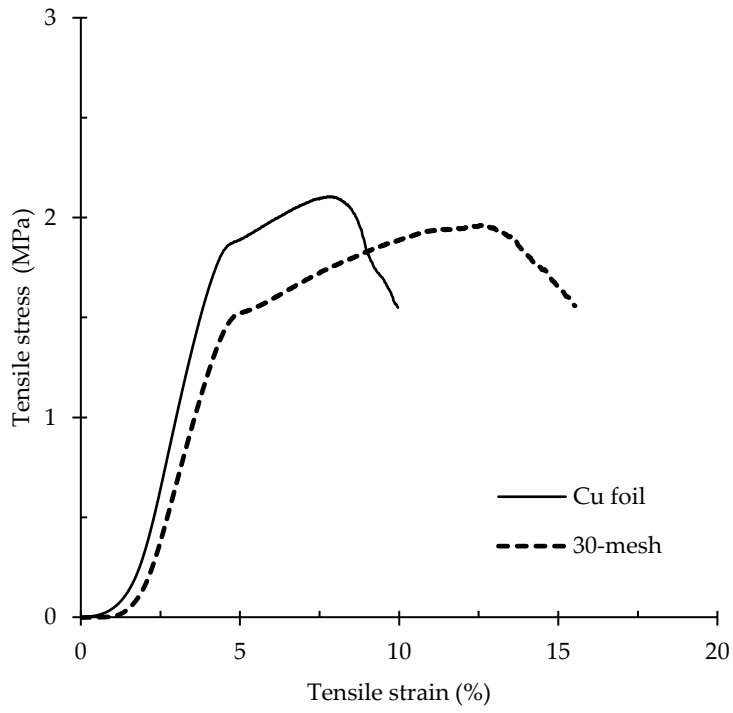
Figure S2. Stress-strain curve of the PLA based 3-layers (PLA-RC-PLA) ENF structures
