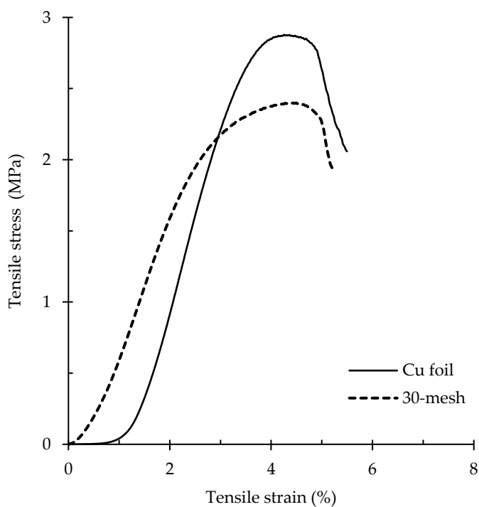
Figure S1. Stress-strain curve of the 2-layers (RC-PLA) ENF structures
