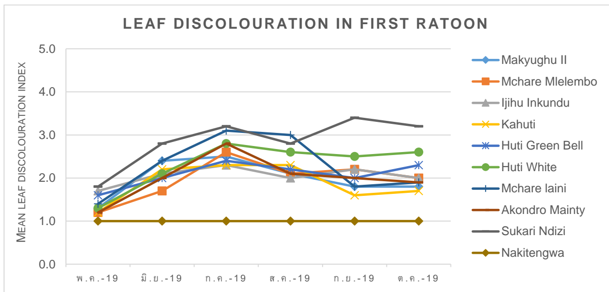
Figure S1. Field evaluation of Mchare cultivars for resistance to Fusarium oxysporum f. sp. ubense race 1 at Arusha, Tanzania. Each time point represents the average leaf discolouration on a rating scale of 1 to 5, with 1 indicating no leaf discolouration, and 5 indicating a dead plant.
