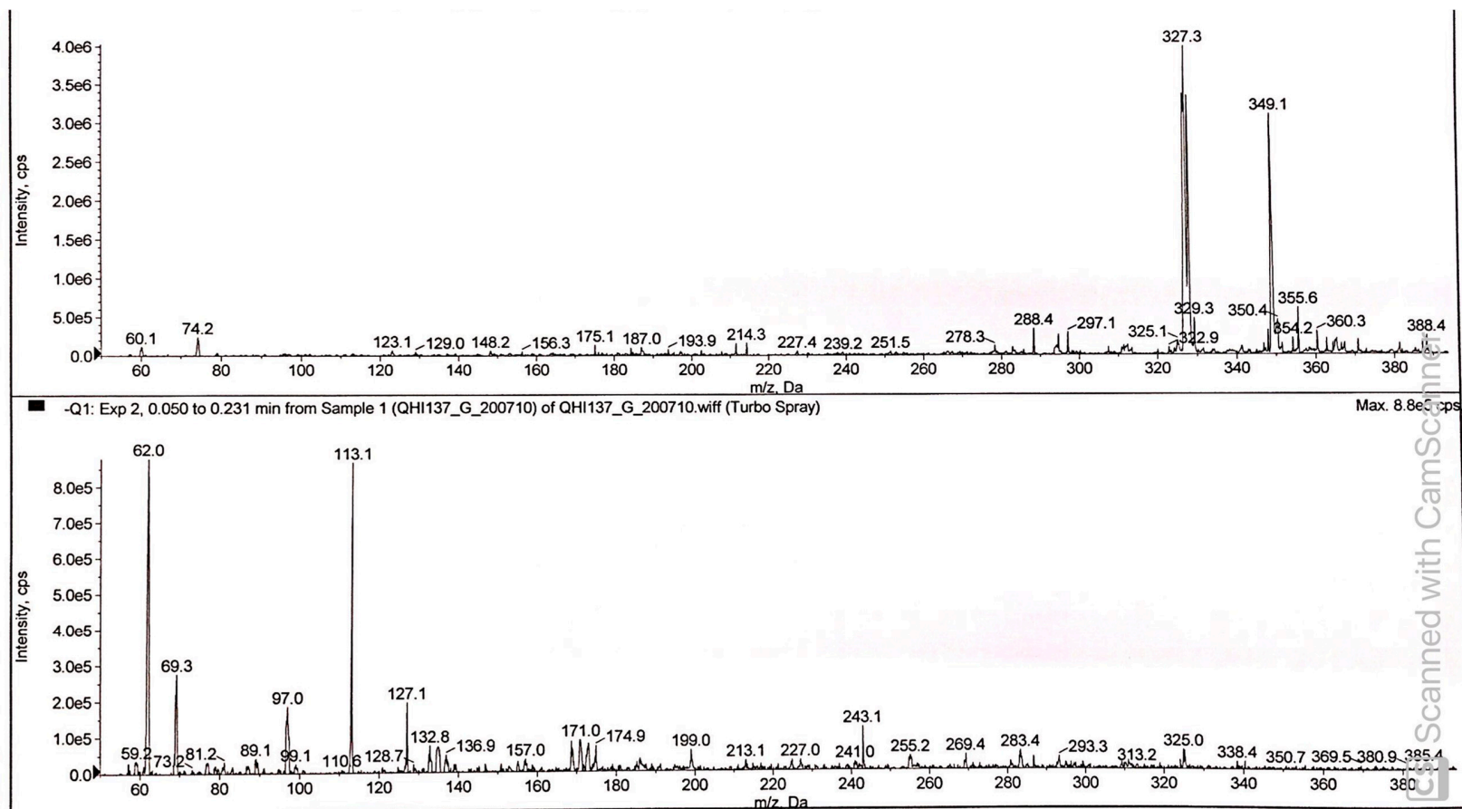
Page S24: Figure S23. HRESIMS spectrum of cichorin F (3).
