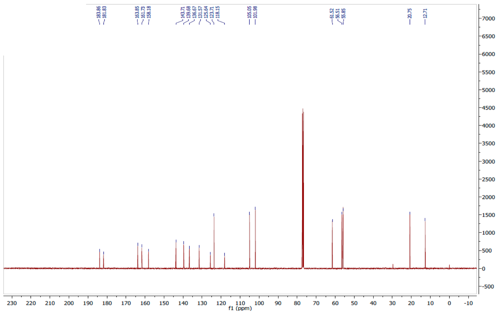
Page S19: Figure S18. ^{13}\text{C} NMR spectrum of cichorin F (3) (400 MHz, \text{CDCl}_3 ).
