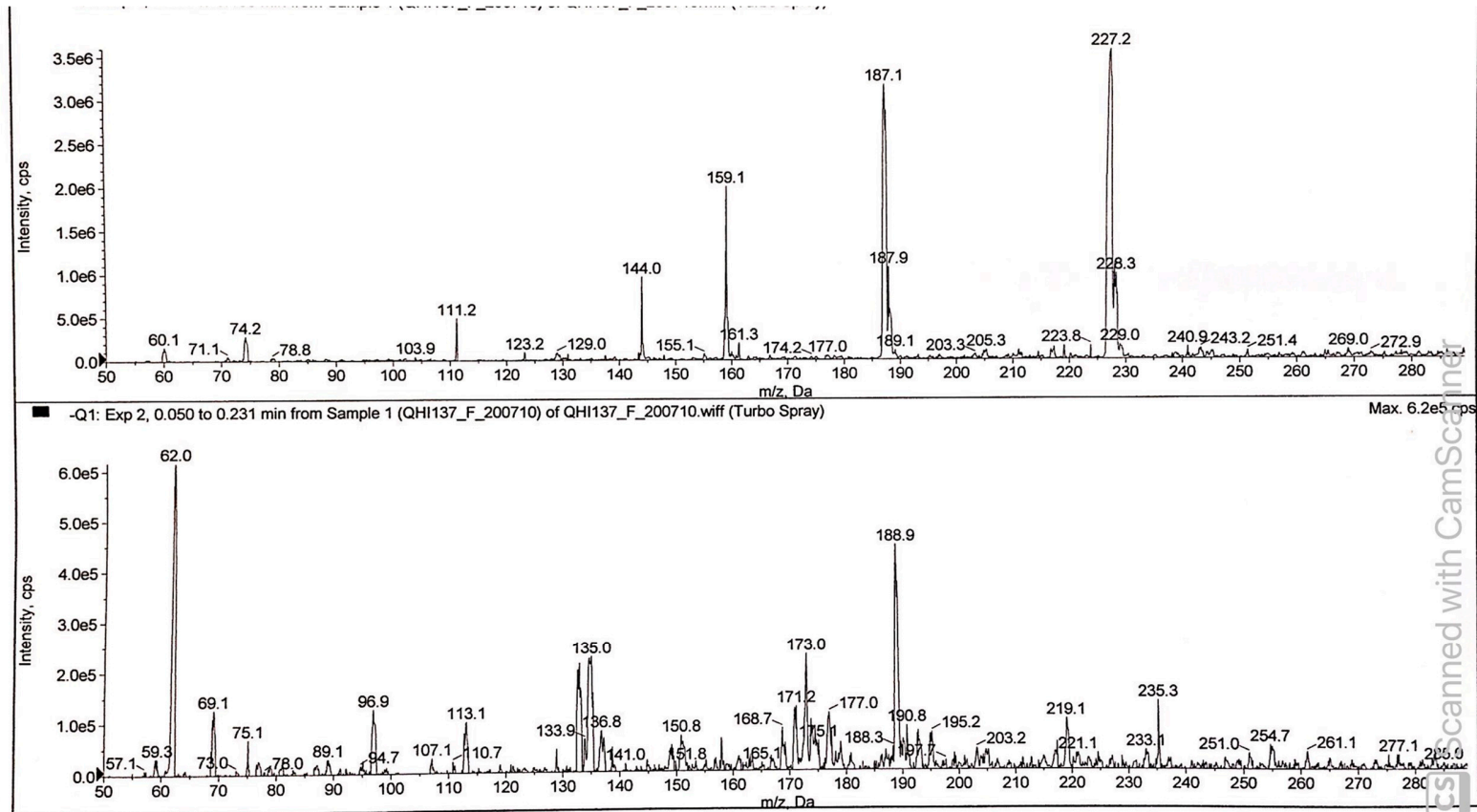
Page S9: Figure S8. ESIMS spectrum of cichorin D (1).
