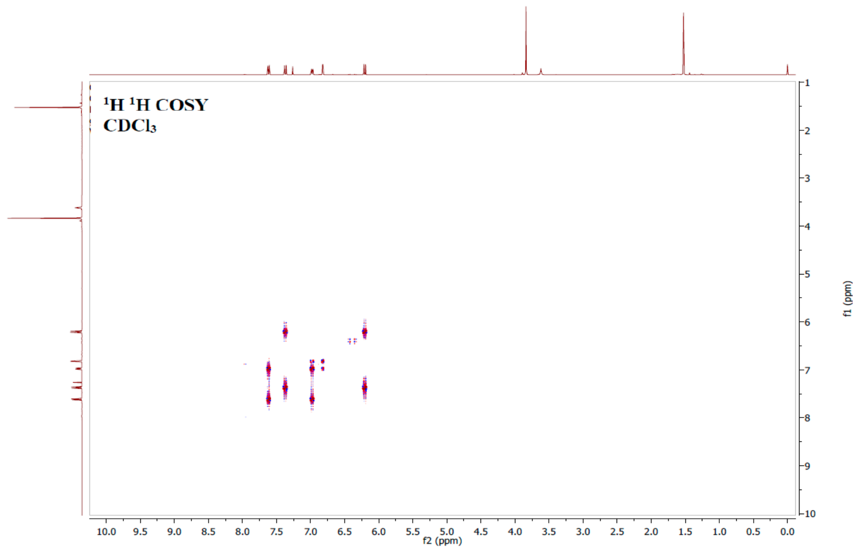
Page S6: Figure S5. COSY spectrum of cichorin D ( 1 ) (400 MHz, CDCl 3 ).
