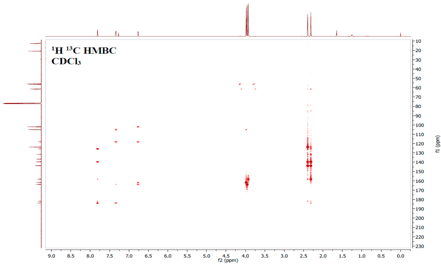
Page S23: Figure S22. HMBC spectrum of cichorin F ( 3 ) (400 MHz, \text{CDCl}_3 ).
