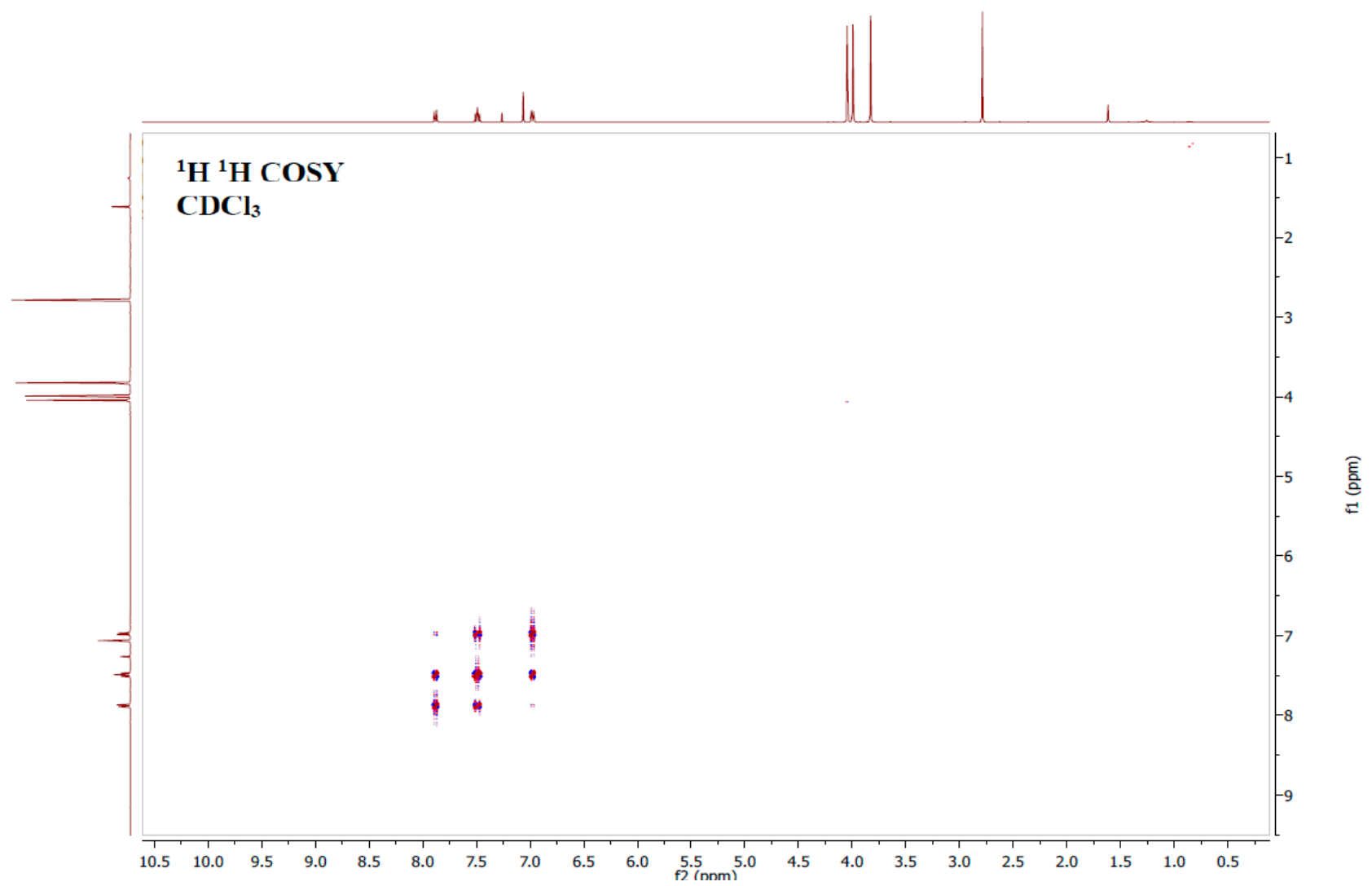
Page S13: Figure S12. COSY spectrum of cichorin E ( 2 ) (400 MHz, \text{CDCl}_3 ).
