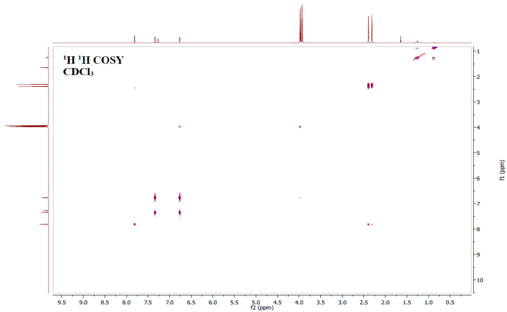
Page S21: Figure S20. COSY spectrum of cichorin F ( 3 ) (400 MHz, CDCl 3 ).
