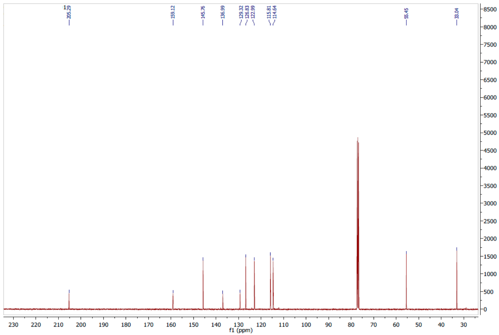
Page S4: Figure S3. ^{13}\text{C} NMR spectrum of cichorin D (1) (400 MHz, \text{CDCl}_3 ).
