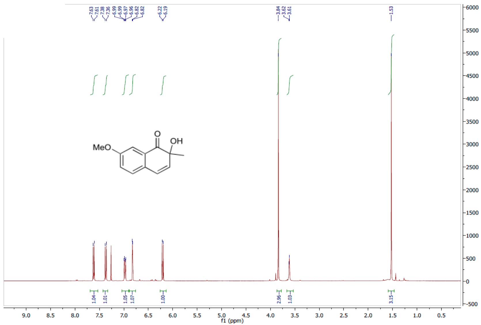
Page S3: Figure S2. 1 H NMR spectrum of cichorin D (1) (400 MHz, CDCl 3 ).
