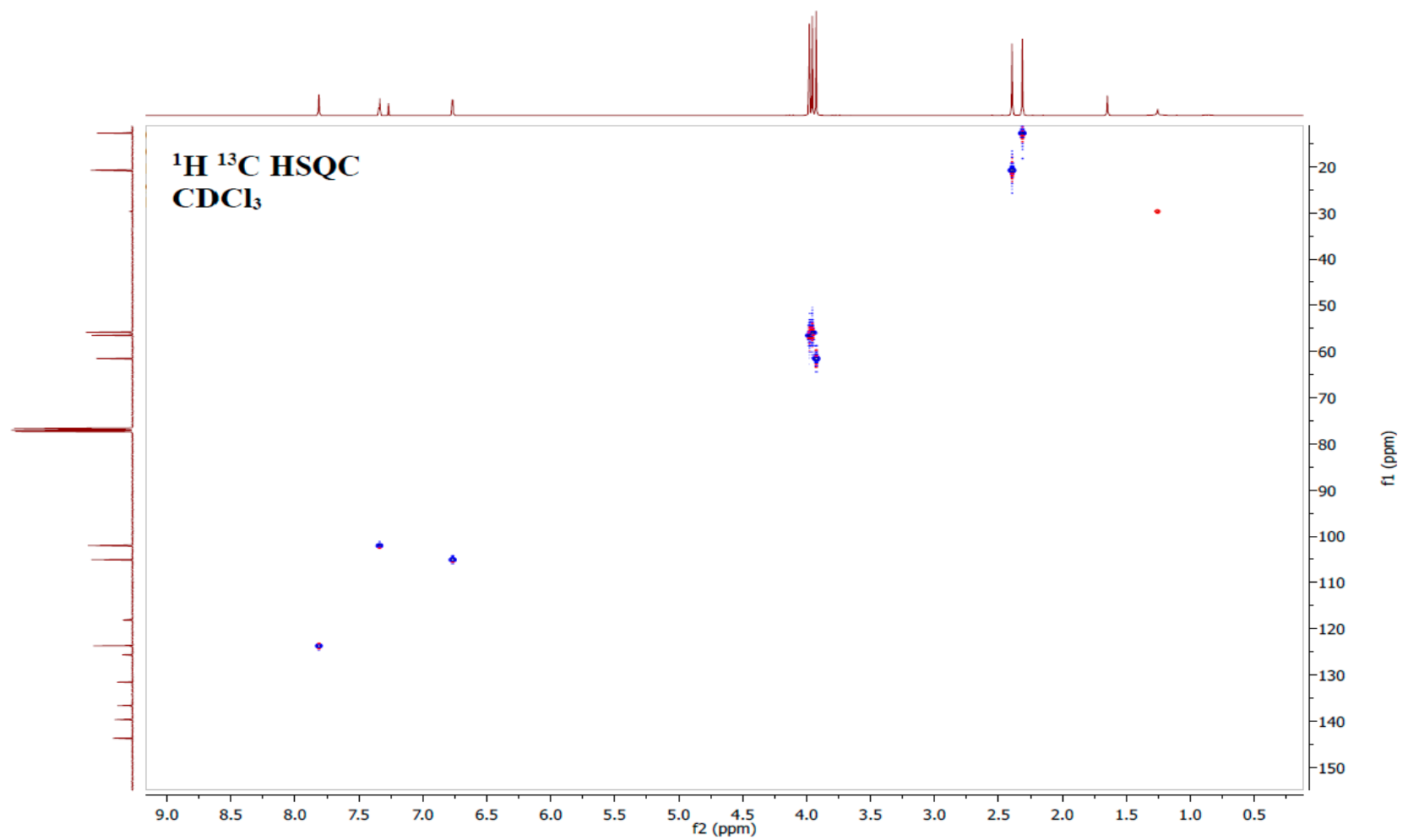
Page S22: Figure S21. HSQC spectrum of cichorin F ( 3 ) (400 MHz, CDCl 3 ).
