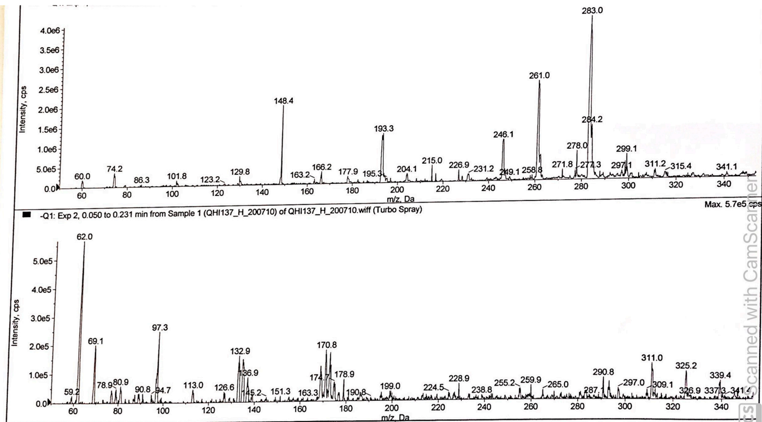
Page S16: Figure S15. ESIMS spectrum of cichorin E (2).
