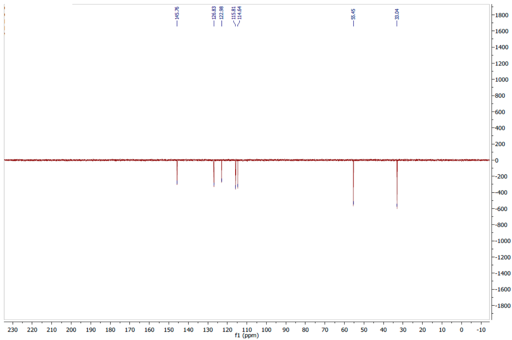
Page S5: Figure S4. DEPT spectrum of cichorin D (1) (400 MHz, CDCl 3 ).
