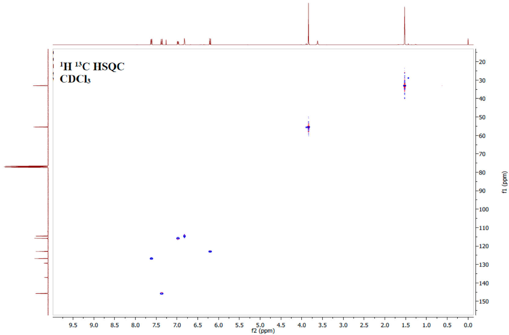
Page S7: Figure S6. HSQC spectrum of cichorin D ( 1 ) (400 MHz, \text{CDCl}_3 ).
