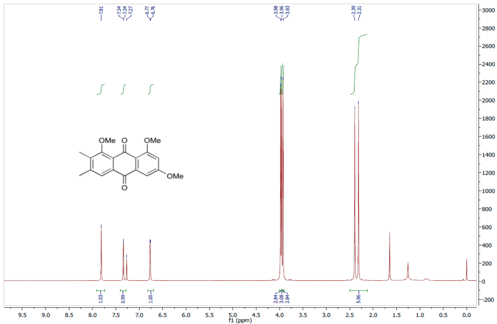
Page S18: Figure S17. 1 H NMR spectrum of cichorin F (3) (400 MHz, CDCl 3 ).
