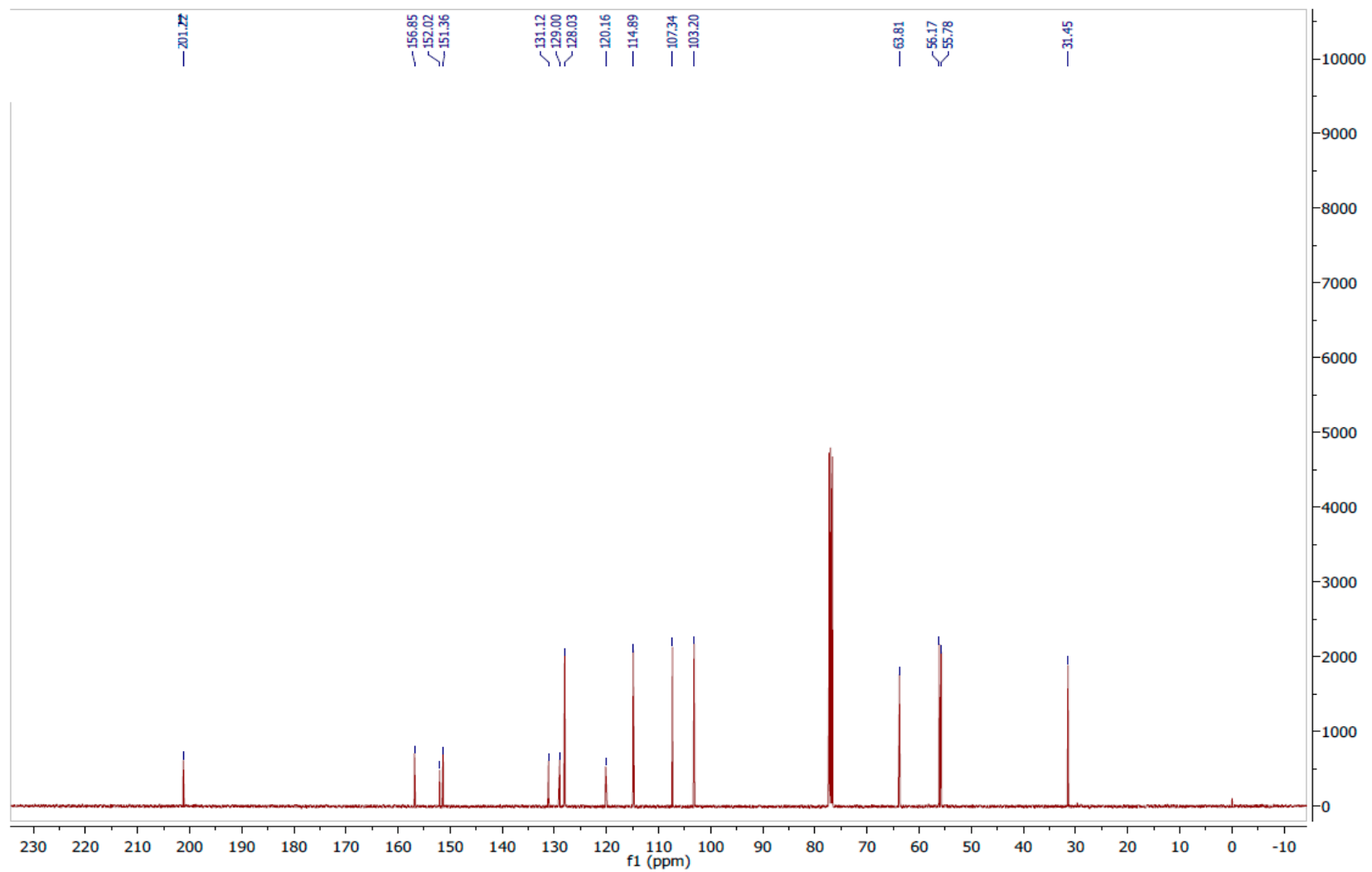
Page S12: Figure S11. ^{13}\text{C} NMR spectrum of cichorin E (2) (400 MHz, \text{CDCl}_3 ).
