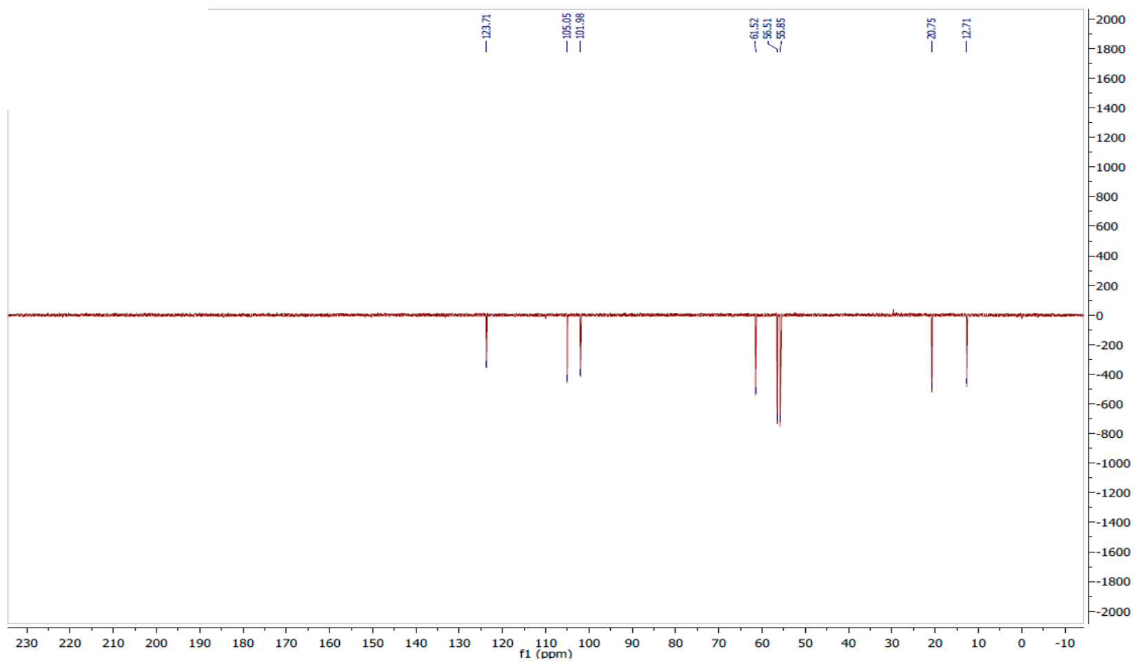
Page S20: Figure S19. DEPT spectrum of cichorin F (3) (400 MHz, CDCl 3 ).
