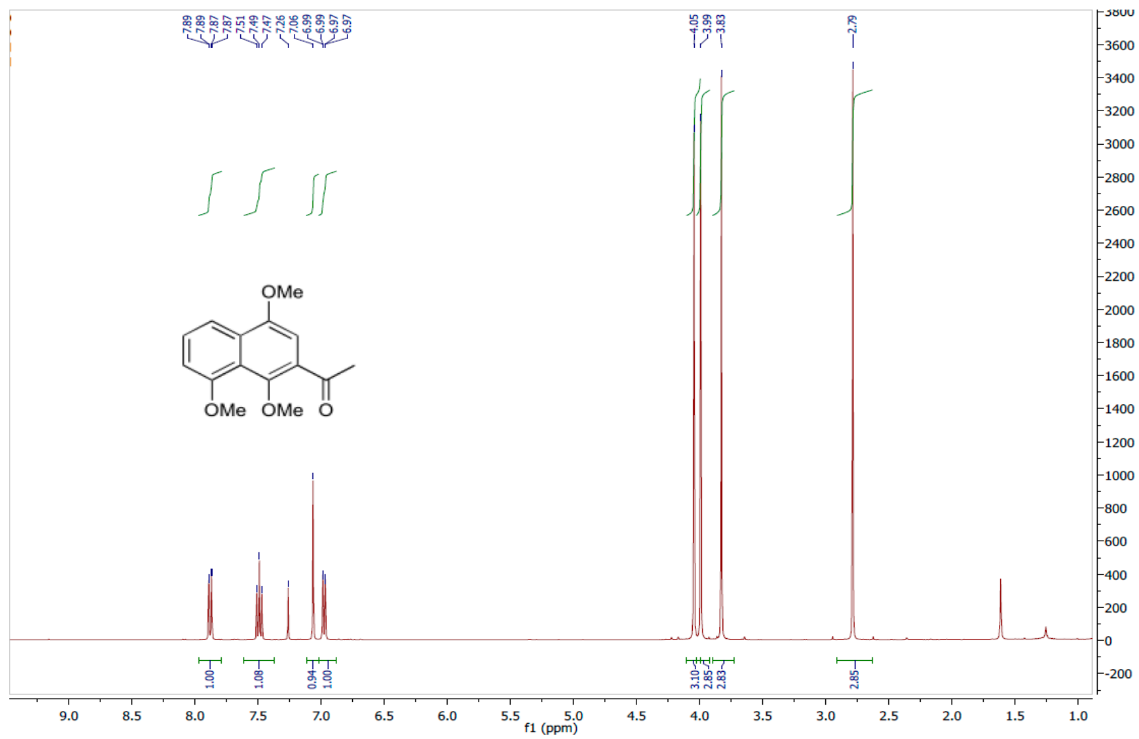
Page S11: Figure S10. 1 H NMR spectrum of cichorin E (2) (400 MHz, CDCl 3 ).
