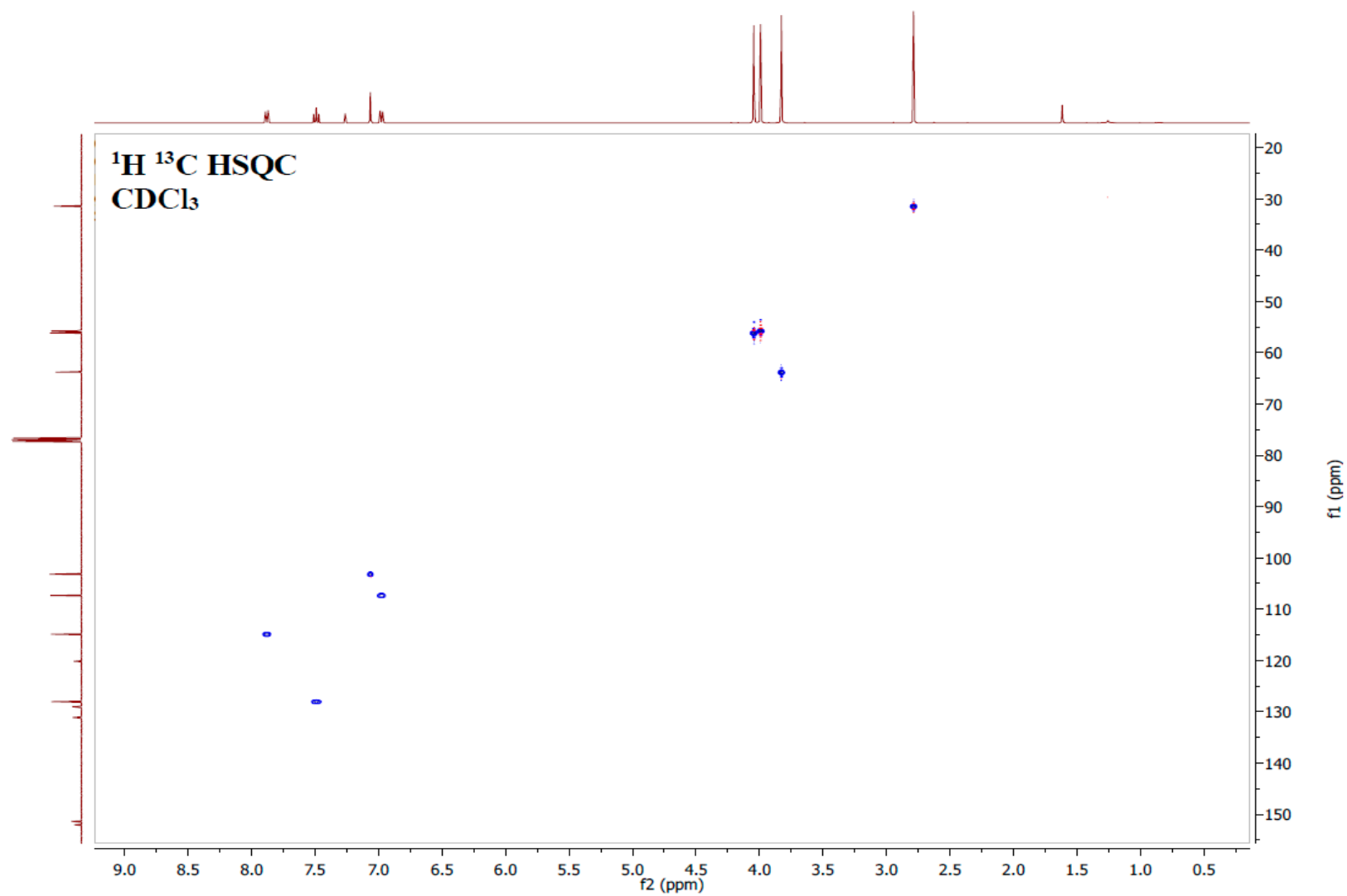
Page S14: Figure S13. HSQC spectrum of cichorin E ( 2 ) (400 MHz, \text{CDCl}_3 ).
