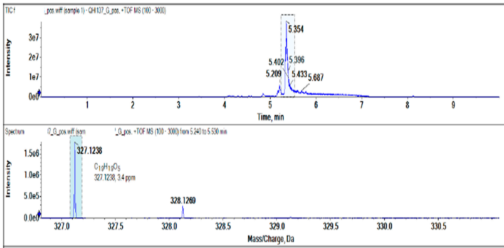
Page S25: Figure S24. HRESIMS spectrum of cichorin F (3).
