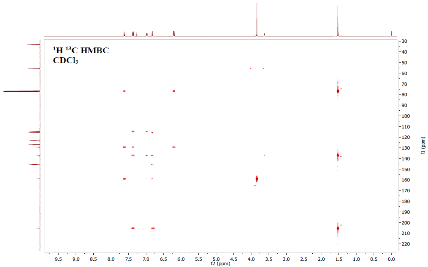
Page S8: Figure S7. HMBC spectrum of cichorin D ( 1 ) (400 MHz, \text{CDCl}_3 ).
