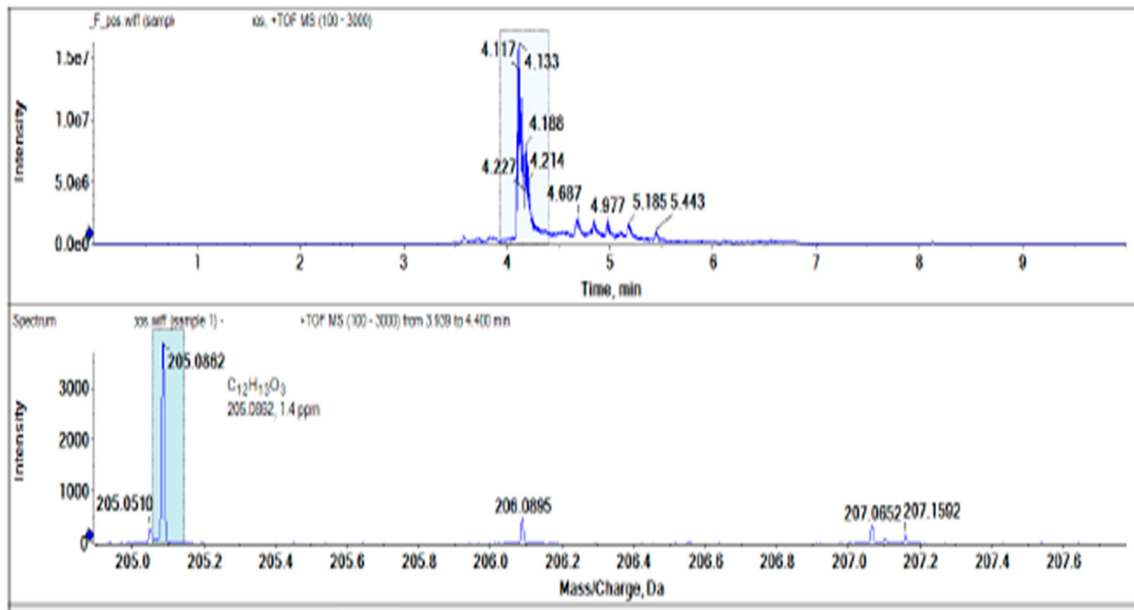
Page S10: Figure S9. HRESIMS spectrum of cichorin D (1).
