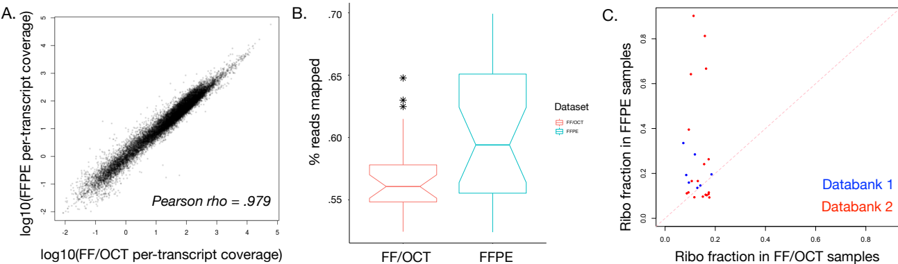
Supplementary Figure 15: Comparison of coverage and read mapping in FFPE vs. FF/OCT replicates. A) Average transcript coverage is highly consistent between replicates. B) Percent reads mapped (mapped reads / total reads) in FFPE vs. FF/OCT replicates. The box plot shows higher mapping rate in FFPE samples. C) Comparison of ribosomal RNA fraction in FFPE and FF/OCT replicate samples. FFPE samples tend to have higher ribosomal RNA content than corresponding FF/OCT samples.
