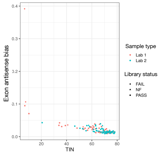
Supplementary Figure 2: Exon bias vs. TIN (A) and GC contents (B). Exon bias correlates negatively with TIN and positively with GC contents.
