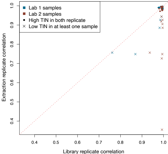
Supplementary Figure 9: Correlations of transcriptional profiles of extraction replicates vs. library replicates. It shows that even when one of the extraction replicates has low quality we can still get highly correlated library replicates from that sample.
