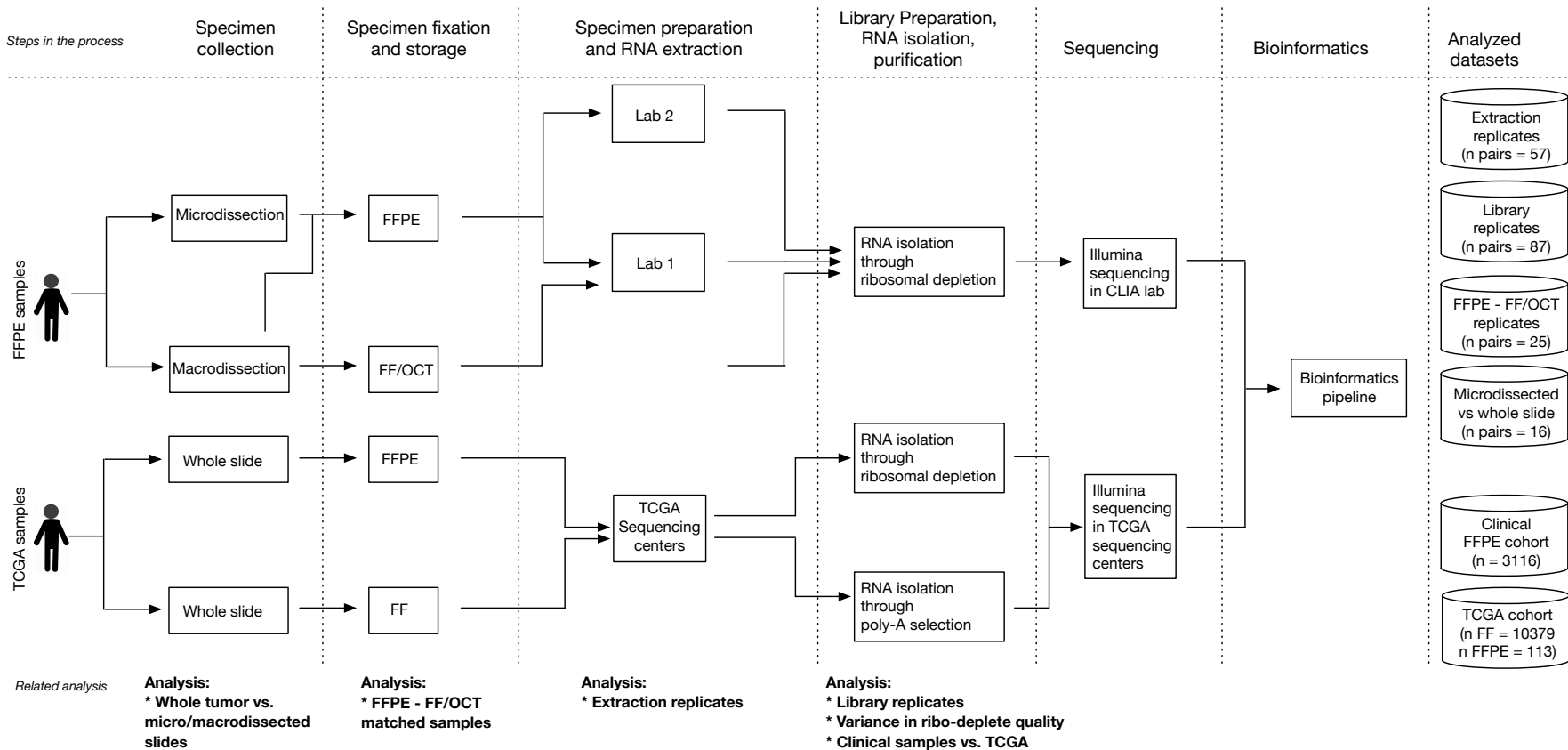
Supplementary Figure 1: Overview of different analyses performed by this study and how they fit into different stages of RNA sequencing process.
