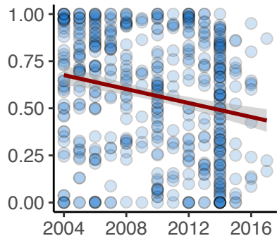
pfprt 76T
