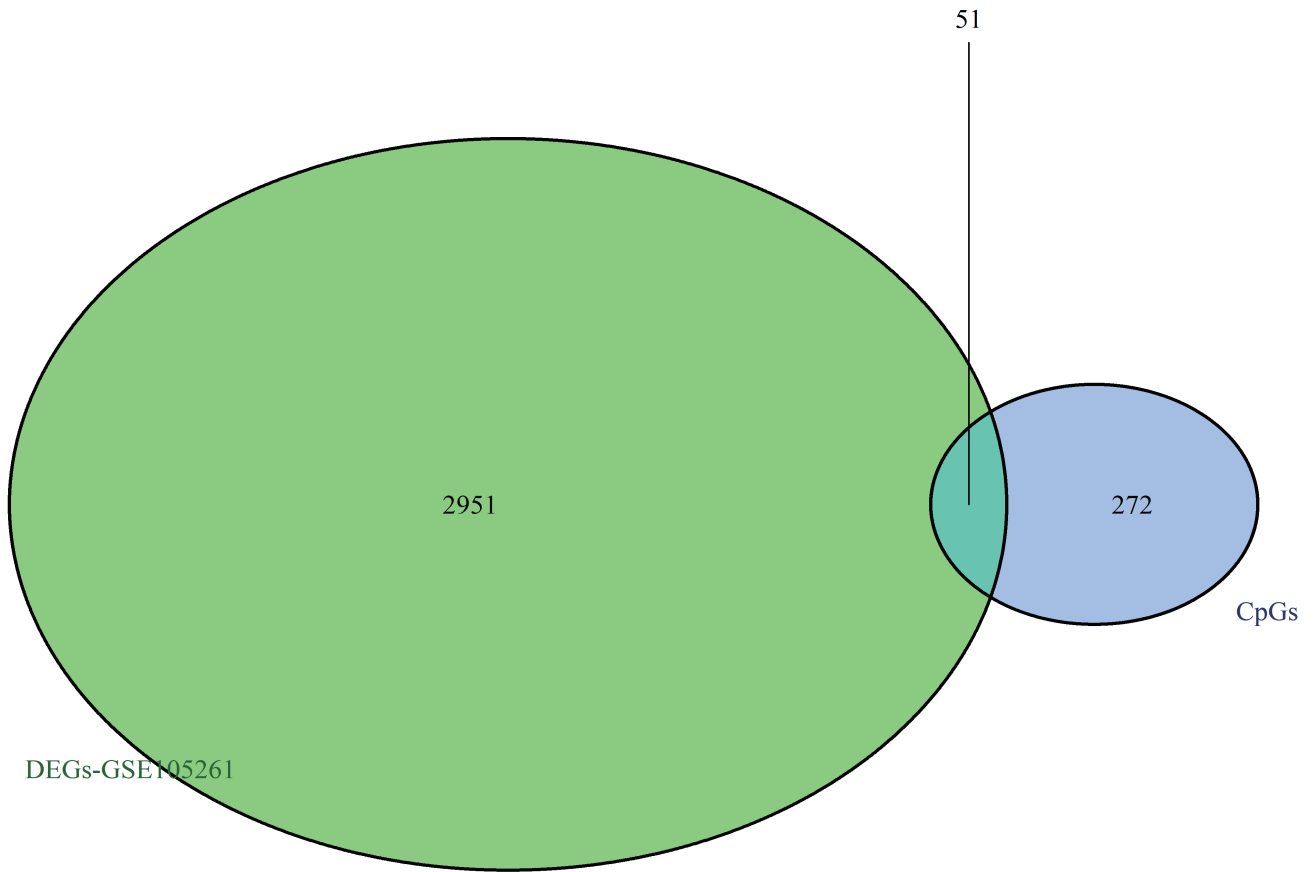
Supplementary figure 1 Venn diagram of overlapping genes among the DMGs based on different regions from GEOdataset GSE105260 and DEGs screened from GEO (GSE105261) dataset.
