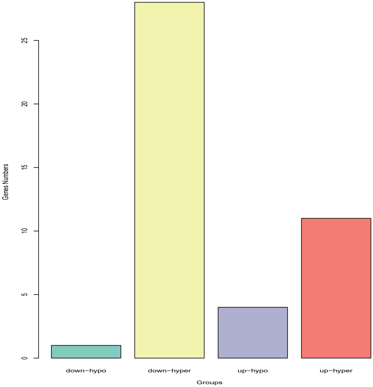
Supplementary figure 5 Characteristics of intersected genes between DEGs from GSE105261 and DMGs based on all region CpGs from GSE105260. a Barplot for four groups of intersected genes. Down-hyper represents downregulated and hyper-methylated genes. Up-hypo represents upregulated and hypo-methylated genes. Up-hyper represents upregulated and hyper-methylated genes. Down-hypo represents downregulated hypo-methylated genes. The y-axis is the number of genes.
