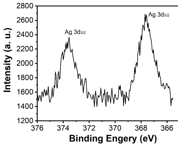
Figure S1. The high-resolution XPS spectrum of Ag 3d.
