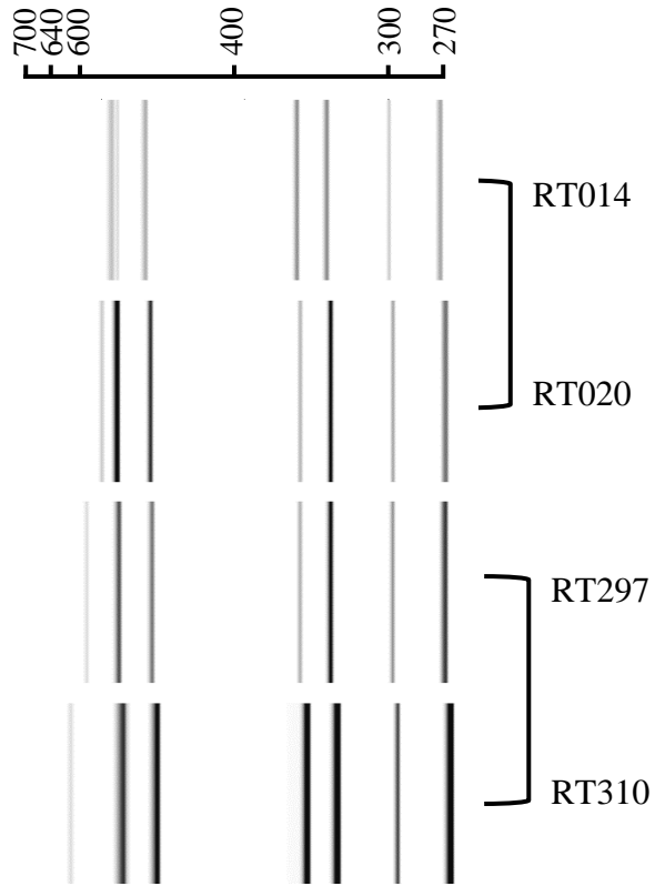
Supplementary Figure 1. PCR RT banding patterns (bps) for RTs 014, 020, 297 and 310.
