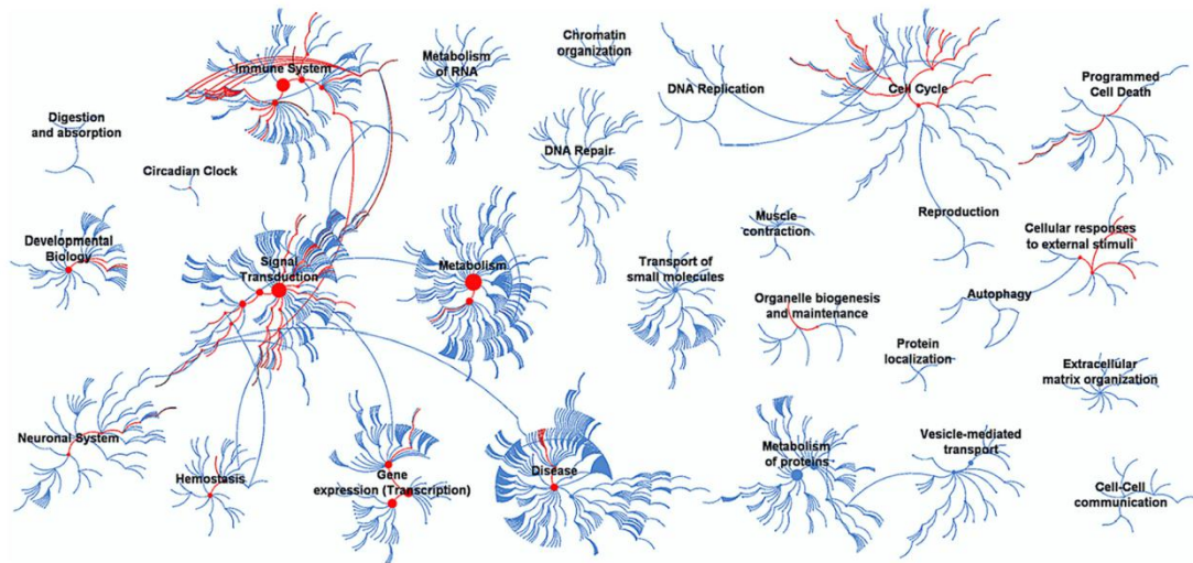
Figure S2. The pathways that NEK2 and its interacting proteins participate in by Reactome database analysis. The red lines in the figure fireworks present the pathways that NEK2 and its interacting proteins may be involved in, and the blue lines present the pathways that NEK2 and its interacting proteins may not be involved in.
