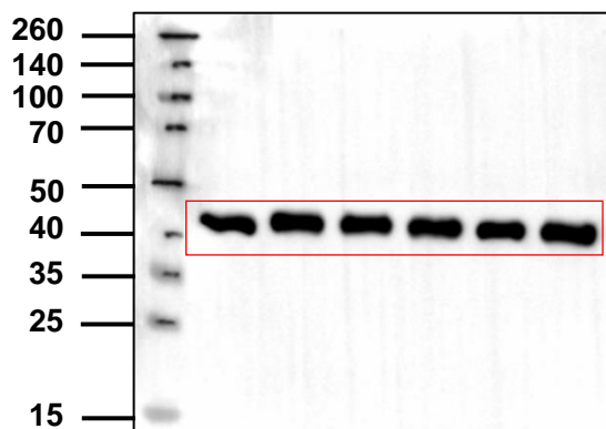
Actin (WWTR1)
