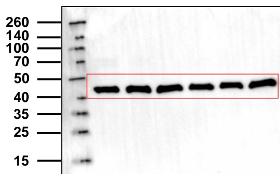
Actin (YAP1)
