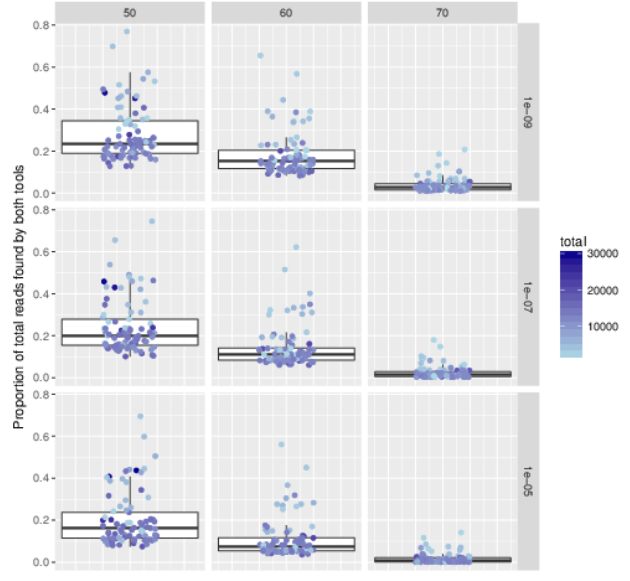
Reads found only by BBmap, for different settings
