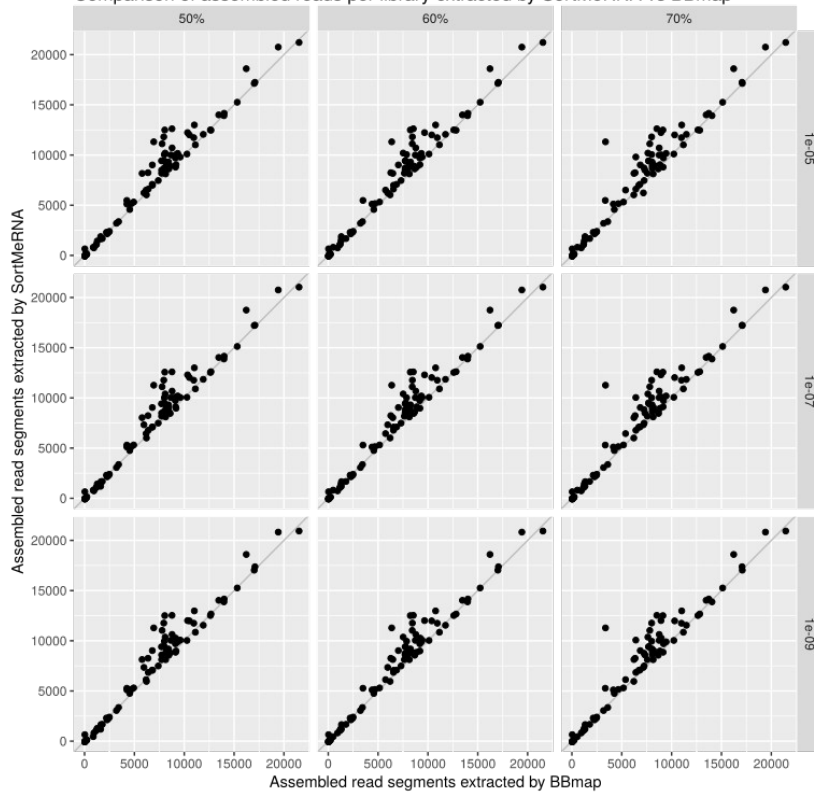
Comparison of assembled reads per library extracted by SortMeRNA vs BBmap
