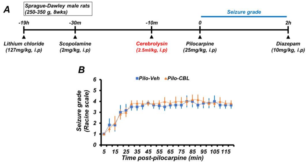
Figure S1. The experimental paradigm used in this study and the seizure grade according to the racine stage. Figure (A) indicates experimental paradigm of pre-treatment cerebrolysin. Cerebrolysin (2.5ml / kg) was administered 10 mins before pilocarpine injection following which, seizure is induced for 2 hours by pilocarpine. Figure (B) is a graph confirming the average score of the seizure grade based on the racine stage after pilocarpine administration. n=6 from each seizure group.
