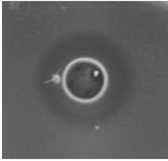
Figure S1. Inhibitory zone result of the non-proteinaceous compound activity against Listeria monocytogenes ATCC19111. To confirm the production of antimicrobial compounds of proteinaceous nature, crystals of pronase E were placed close to the edge of the wells.
