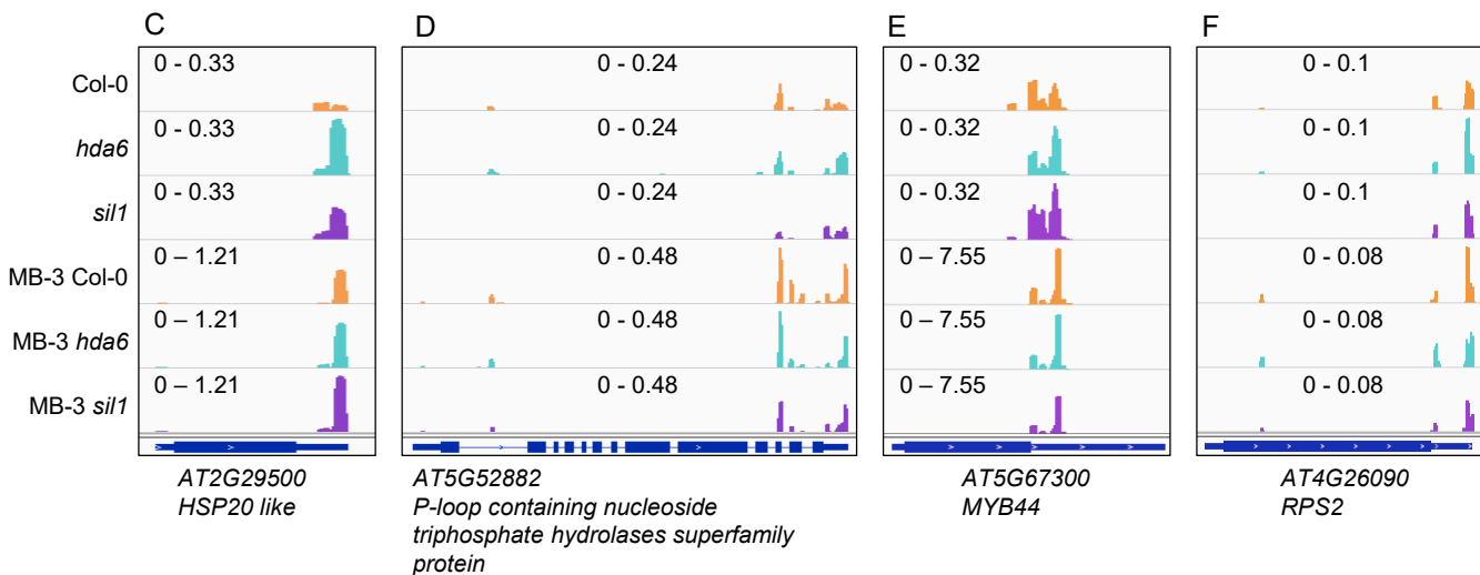
Supplemental Fig S4. Gene Ontology enrichments of genes with up- and down- regulated poly(A) sites. A and B, GO enrichments of genes with up- and down- regulated poly(A) sites, respectively. C-F, PAT-seq tracks of example APA genes. Sequencing coverage scales are indicated on each panel.
